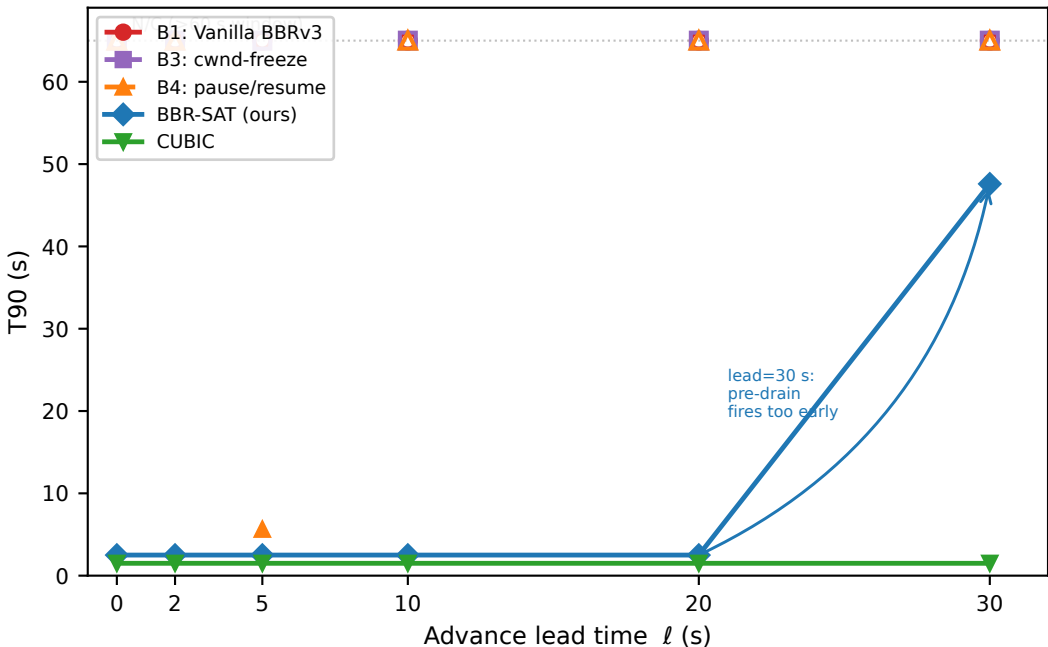
T90 vs lead time — LEO→GEO, T_{\text{HO}} = 30\text{ s}
