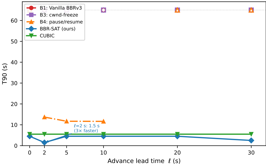
T90 vs lead time — LEO→GEO, T_{HO} = 30 s, 1\times BDP cap
