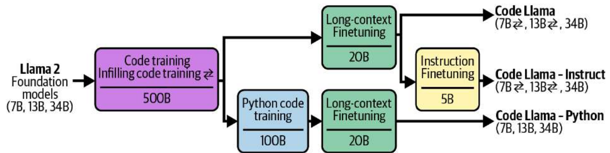
Figure 7-1. Different finetuning techniques used to make different Code Llama models. Image from the Rozière et al. (2024). Adapted from an original image licensed under CC BY 4.0.
