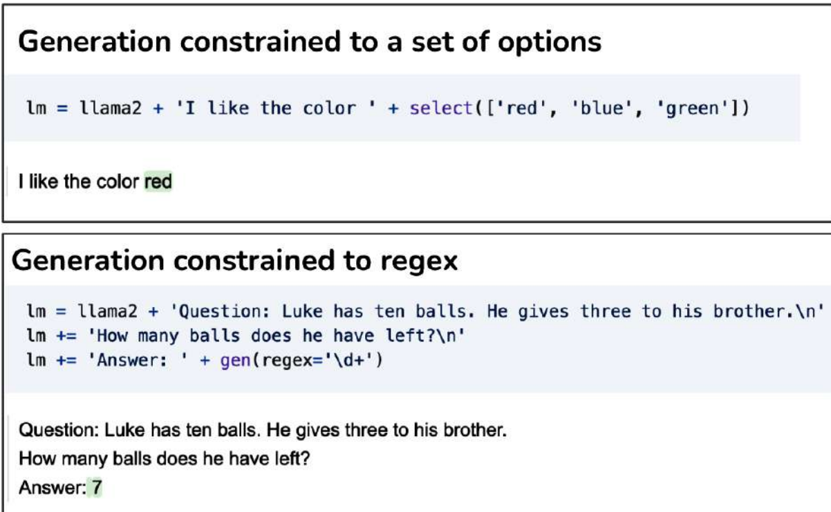
Figure 2-20. Using guidance to generate constrained outputs.
