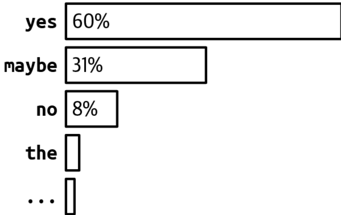
Figure 2-18. Example token probabilities.
