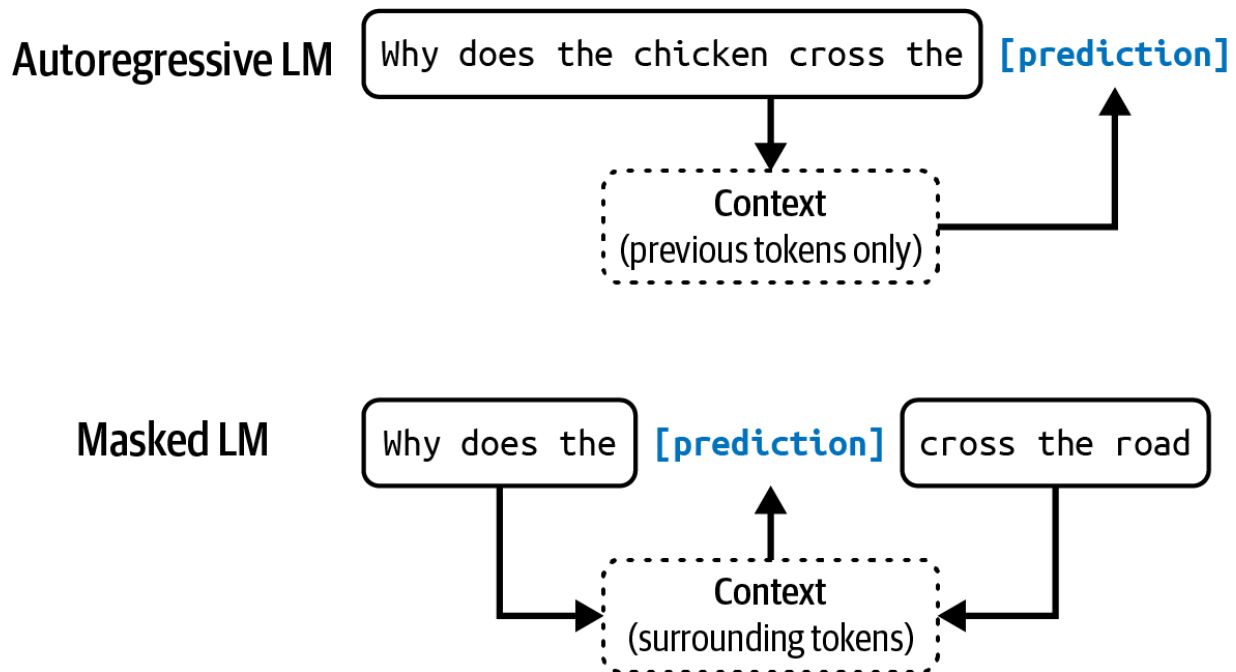
Figure 1-2. Autoregressive language model and masked language model.
