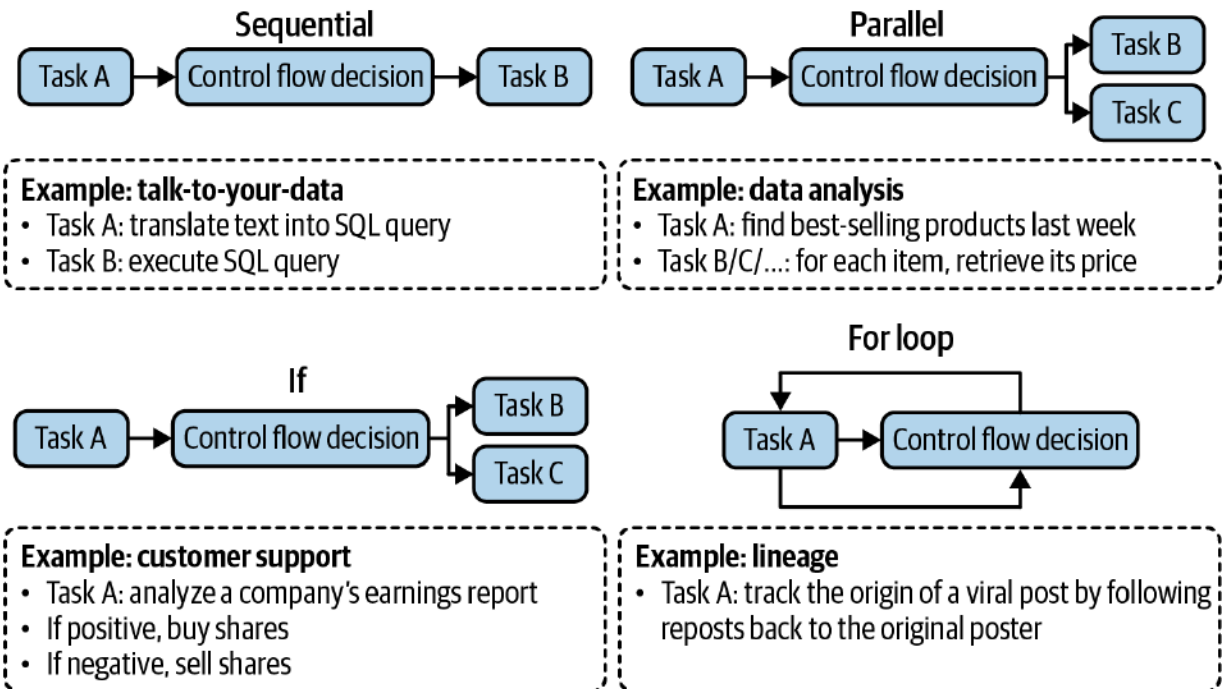
Figure 6-11. Examples of different orders in which a plan can be executed.
