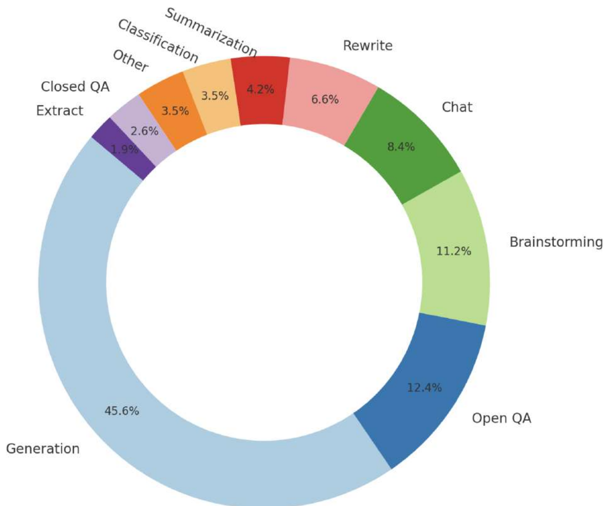
Figure 2-12. The distribution of prompts used to finetune InstructGPT. The graph is created based on the numbers from the OpenAI paper.
