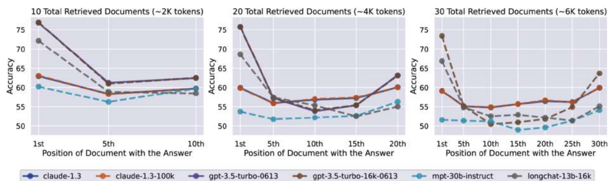
Figure 5-4. The effect of changing the position of the inserted information in the prompt on models' performance. Lower positions are closer to the start of the input context.
