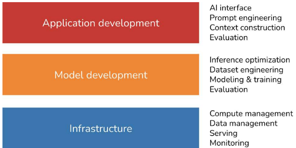
Figure 1-14. Three layers of the AI engineering stack.
