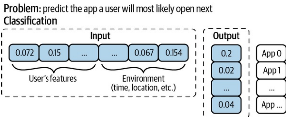
Figure 2-5. Given the problem of predicting the app a user will most likely open next, you can frame it as a classification problem. The input is the user's features and environment's features. The output is a distribution over all apps on the phone.
