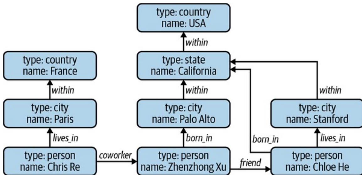
Figure 3-5. An example of a simple graph database
