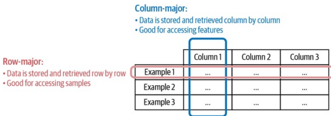
Figure 3-1. Row-major versus column-major formats
