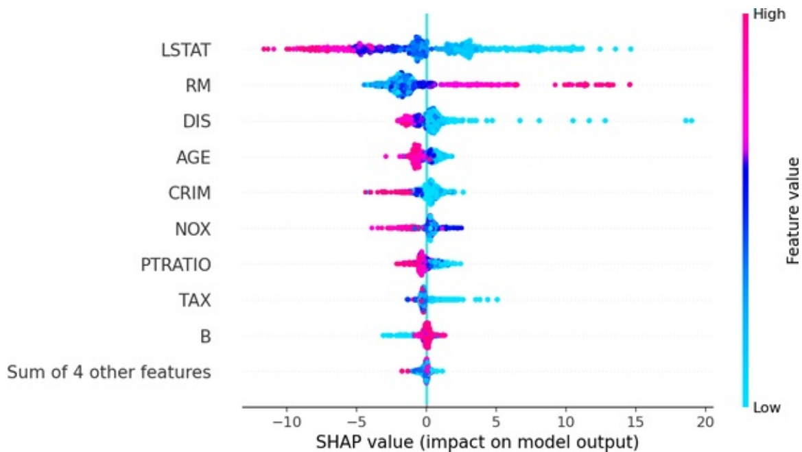
Figure 5-9. How much each feature contributes to a model, measured by SHAP. The feature LSTAT has the highest importance. Source: Scott Lundberg
