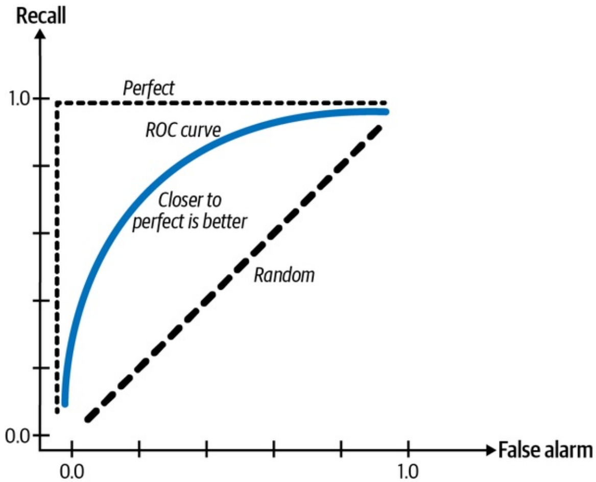
Figure 4-9. ROC curve
