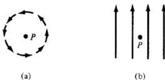
Figure Determining the sense of d\mathbf{l} and d\mathbf{S} involved in Stokes's theorem.
