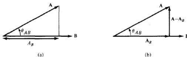
Figure Components of \mathbf{A} along \mathbf{B} : (a) scalar component A_B , (b) vector component \vec{A}_B .
