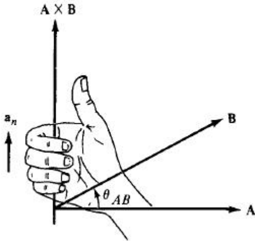
Figure The cross product of A and B is a vector with magnitude equal to the area of the parallelogram and direction as indicated.
