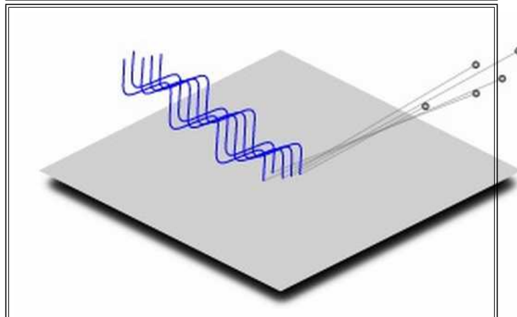
Blue light ejects photoelectrons with more energy than green light (even if it is very dim).
