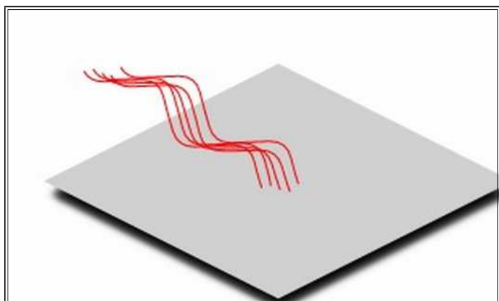
Red light does not eject photoelectrons (even if it is very bright).
