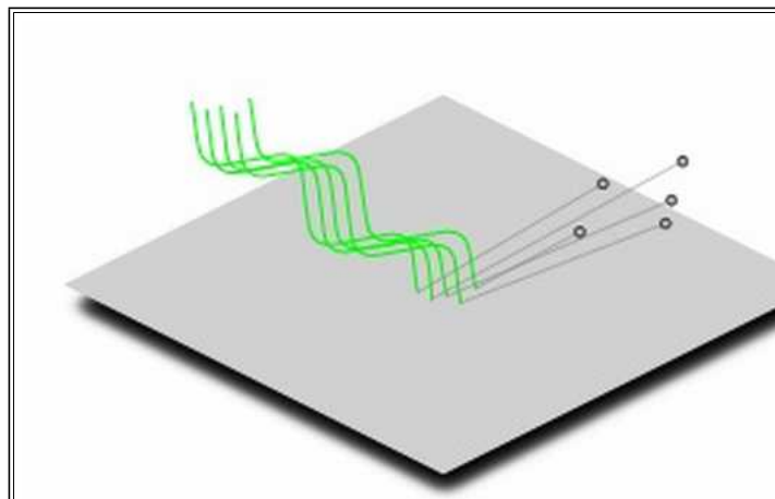
Green light does eject photoelectrons (even if it is very dim).
