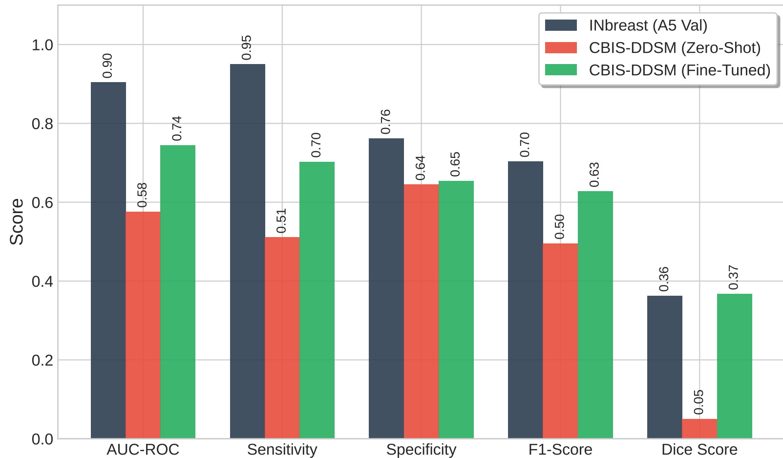
Cross-Dataset Generalisation: INbreast vs CBIS-DDSM
