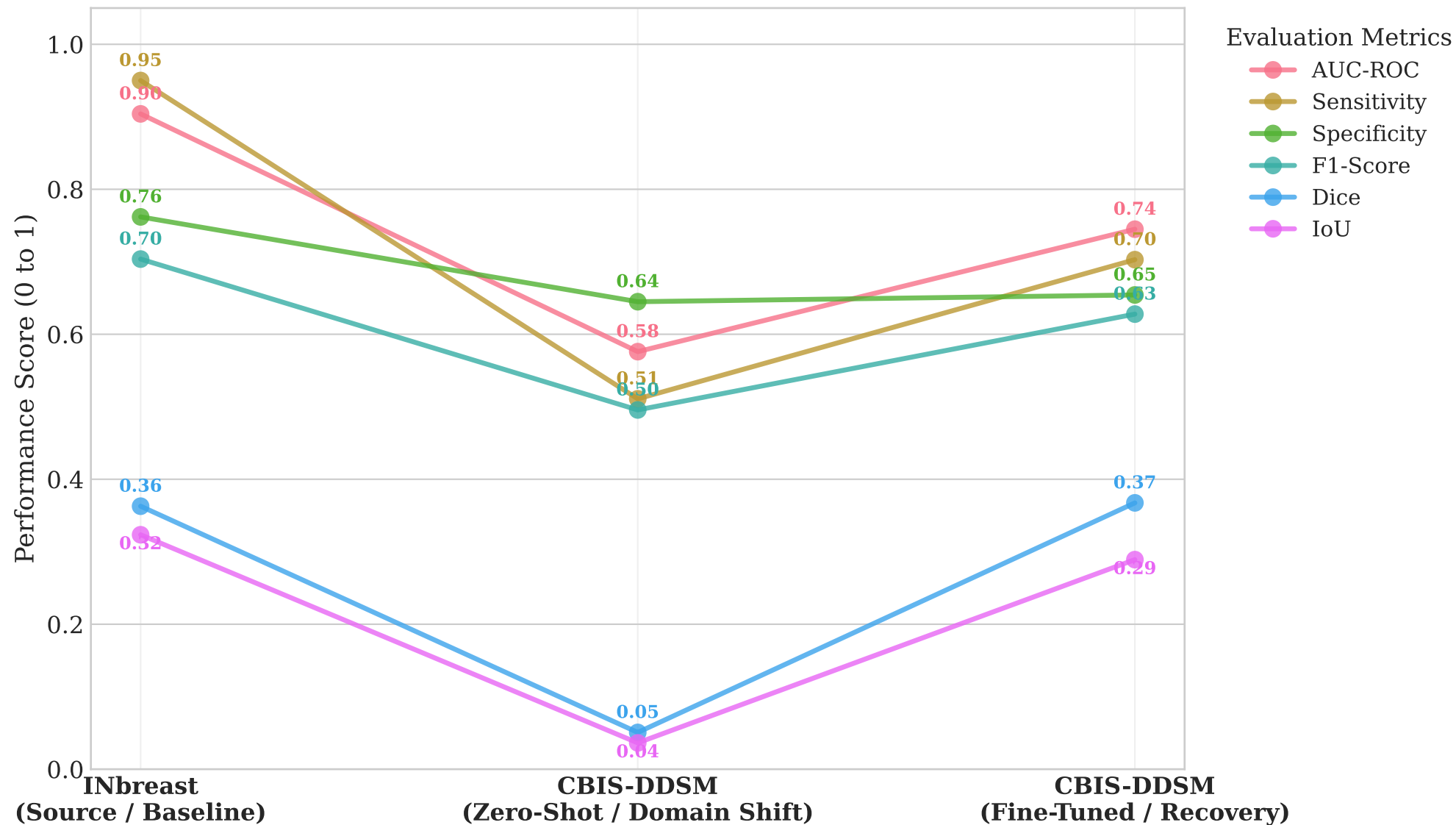
Model Performance Trajectory: Domain Shift and Fine-Tuning Recovery
