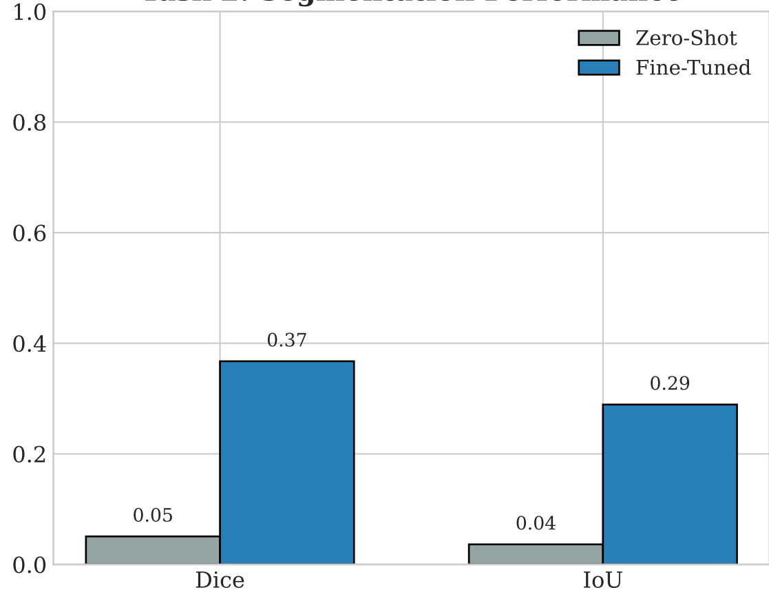
Task 2: Segmentation Performance
