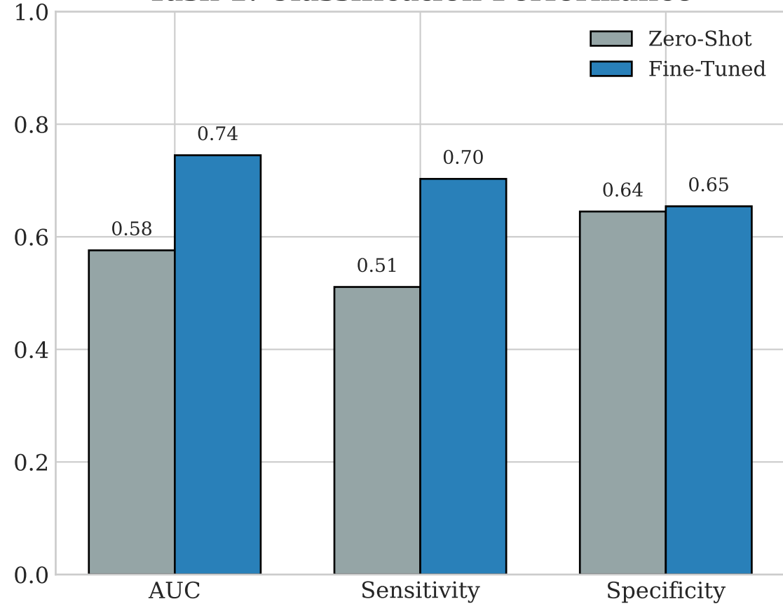
Task 1: Classification Performance
