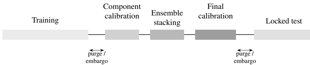
Figure 2: Chronological development protocol. Internal calibration and stacking roles are separated in time, and the locked test is not used for model fitting or threshold selection.
