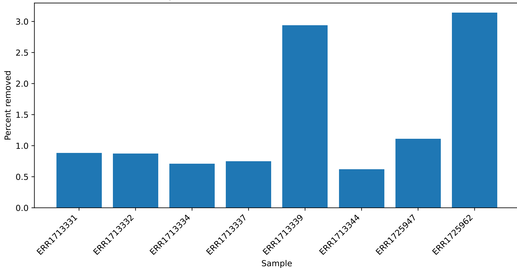
Stage 3.3 Bowtie2: Host/contaminant removal rate
