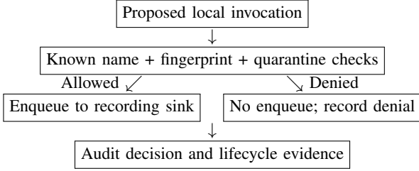
Figure 2. Decision flow. The allowed branch goes directly to its sink; the denied branch never joins the allowed execution path. Quarantine is registry state.
