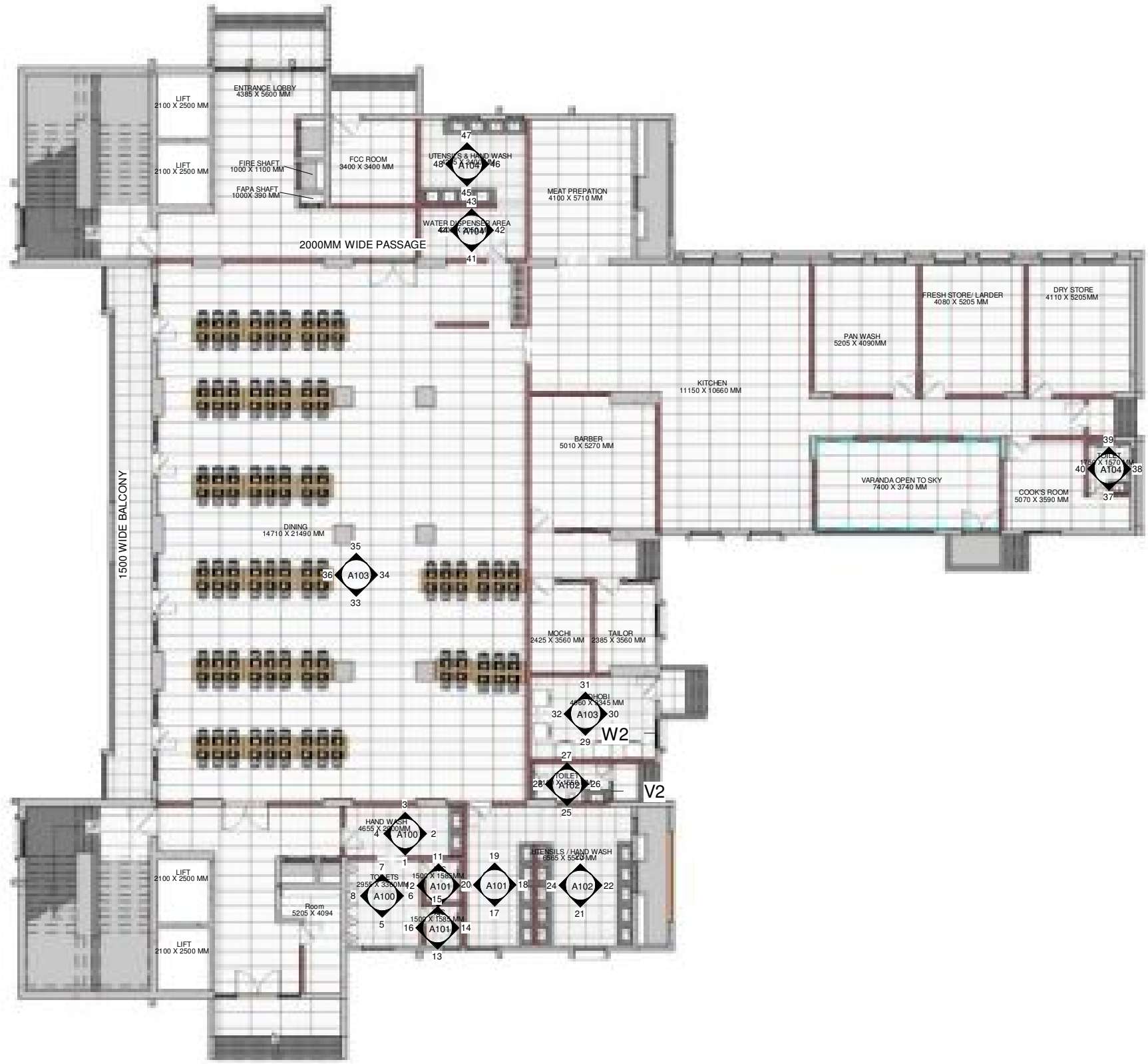
0 CDO GROUND FLOOR PLAN Copy 1 1 : 200
