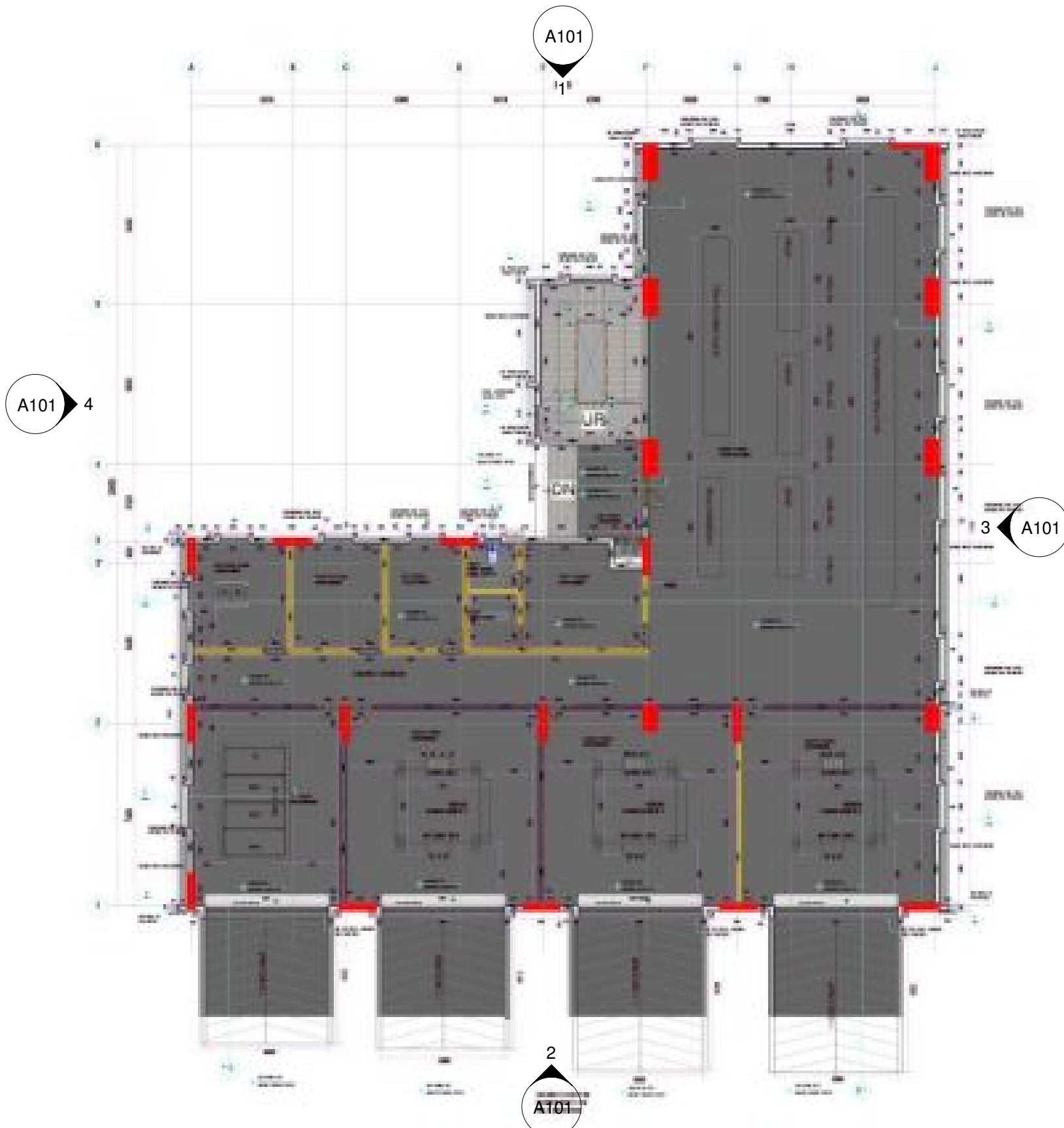
3 GROUND FLOOR LEVEL 1 : 200
