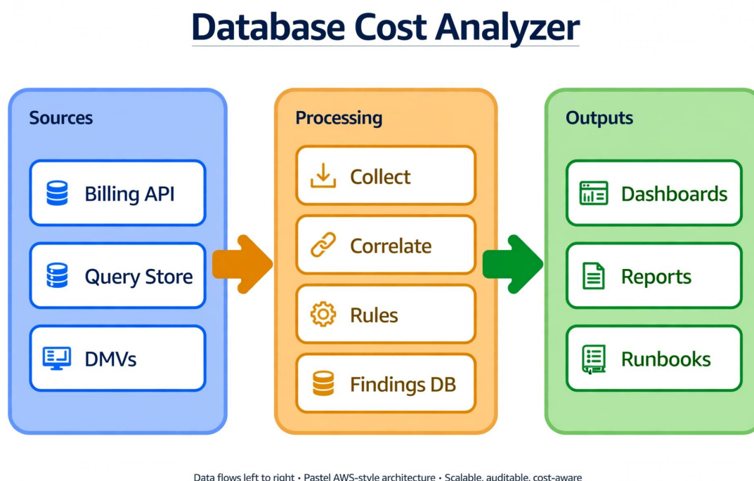
Figure 29.1 — Database cost analyzer. Three zones turn raw billing and telemetry into prioritized, trackable savings findings.
