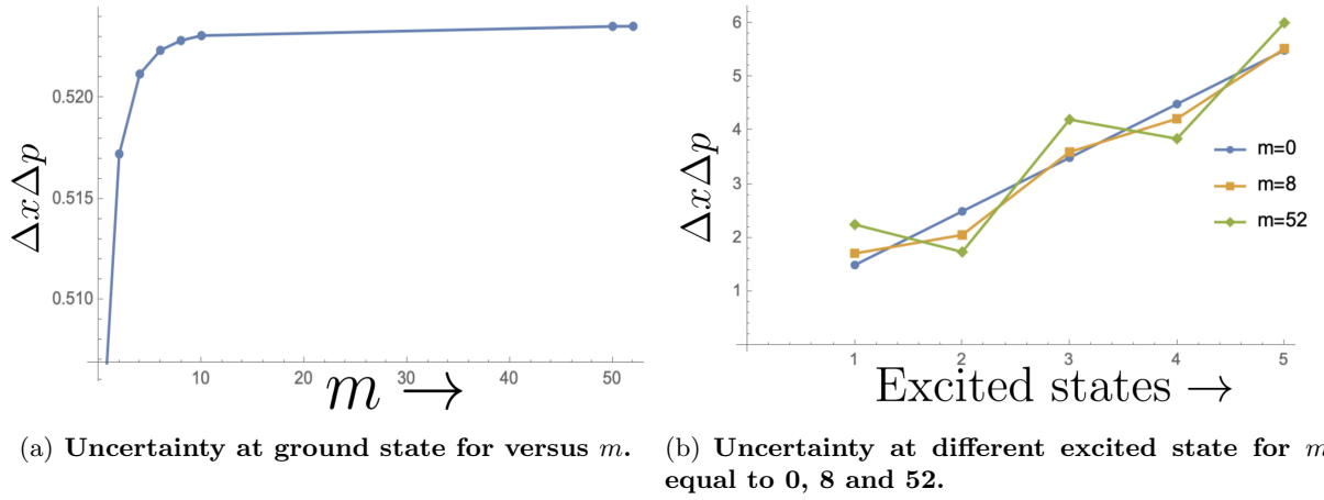
Figure 6: Uncertainty trends with increasing m and n .
