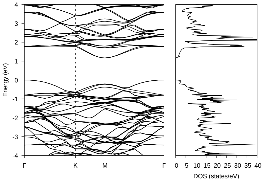
BN/MoS2 Bandstructure and DOS
