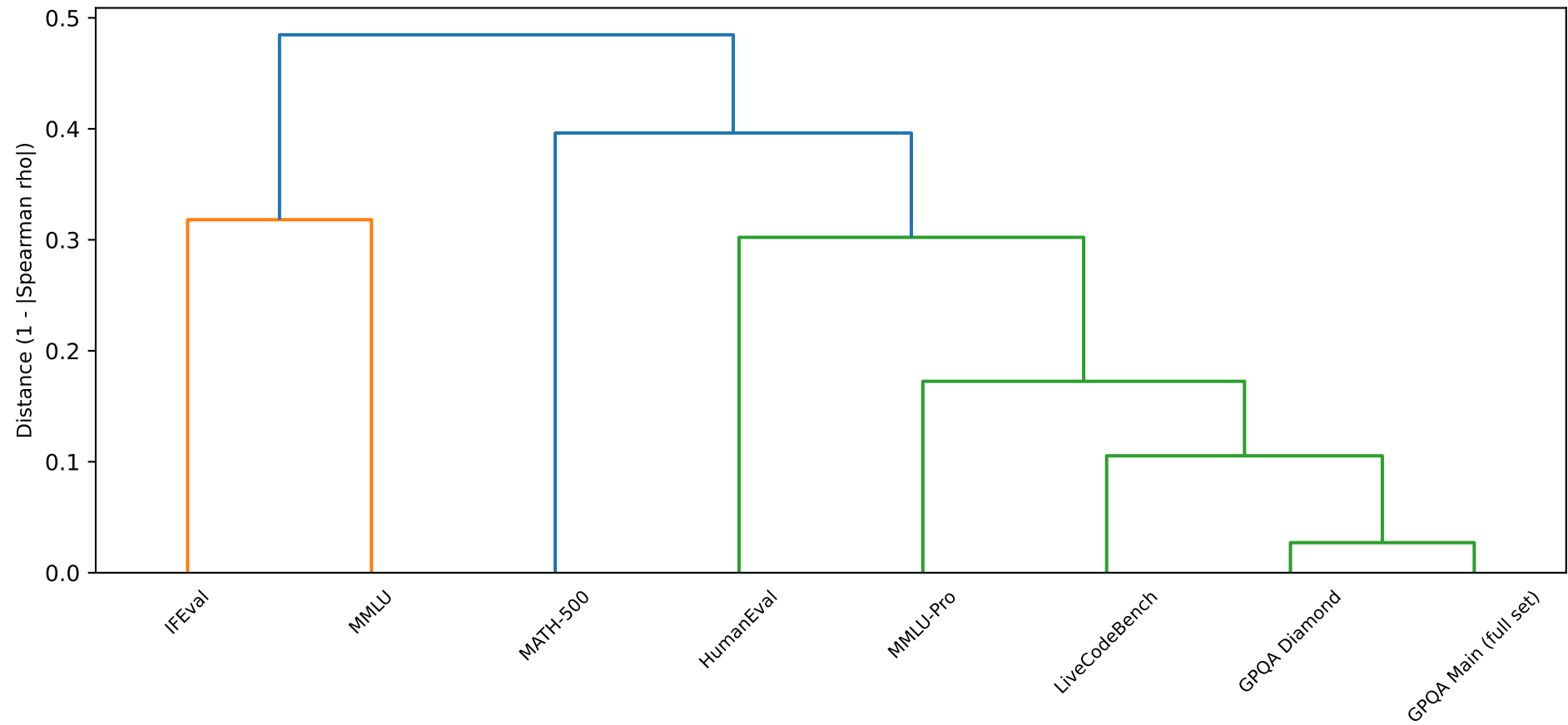
Correlation-Based Hierarchical Clustering
