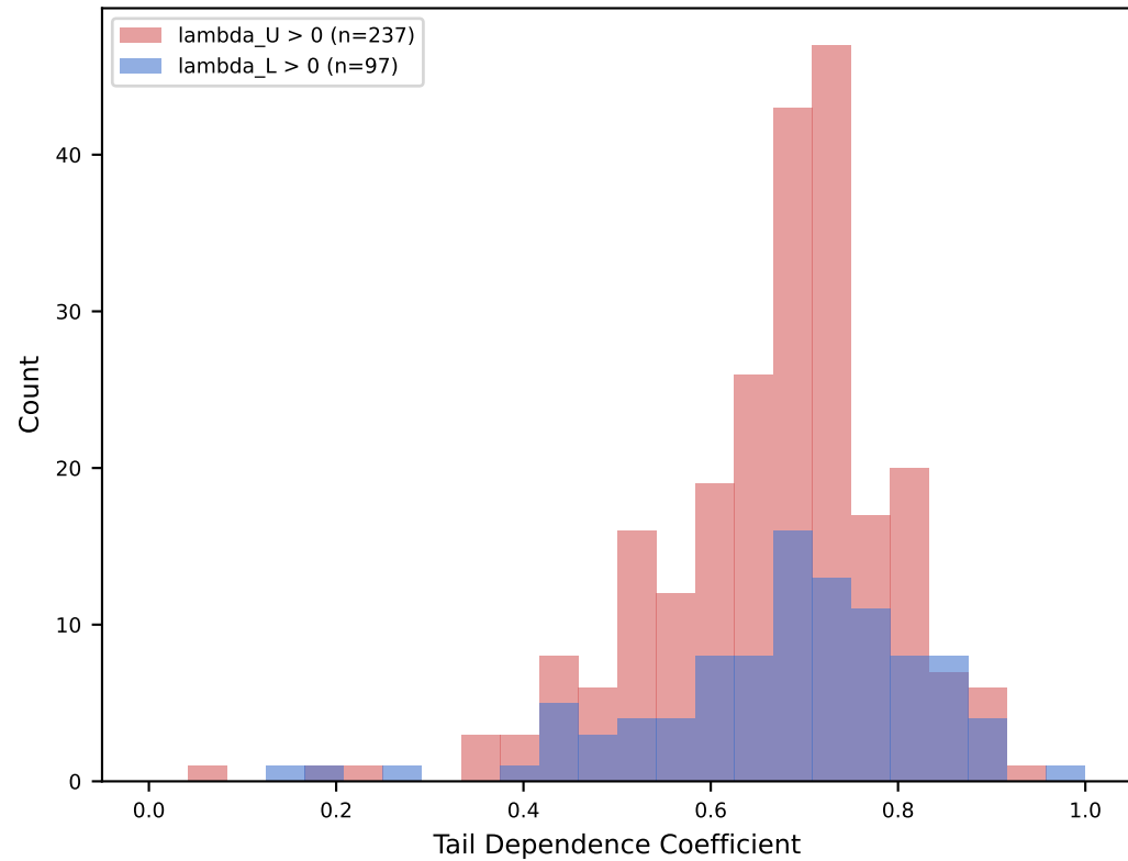
(b) Distribution of Non-Zero Tail Dependence
