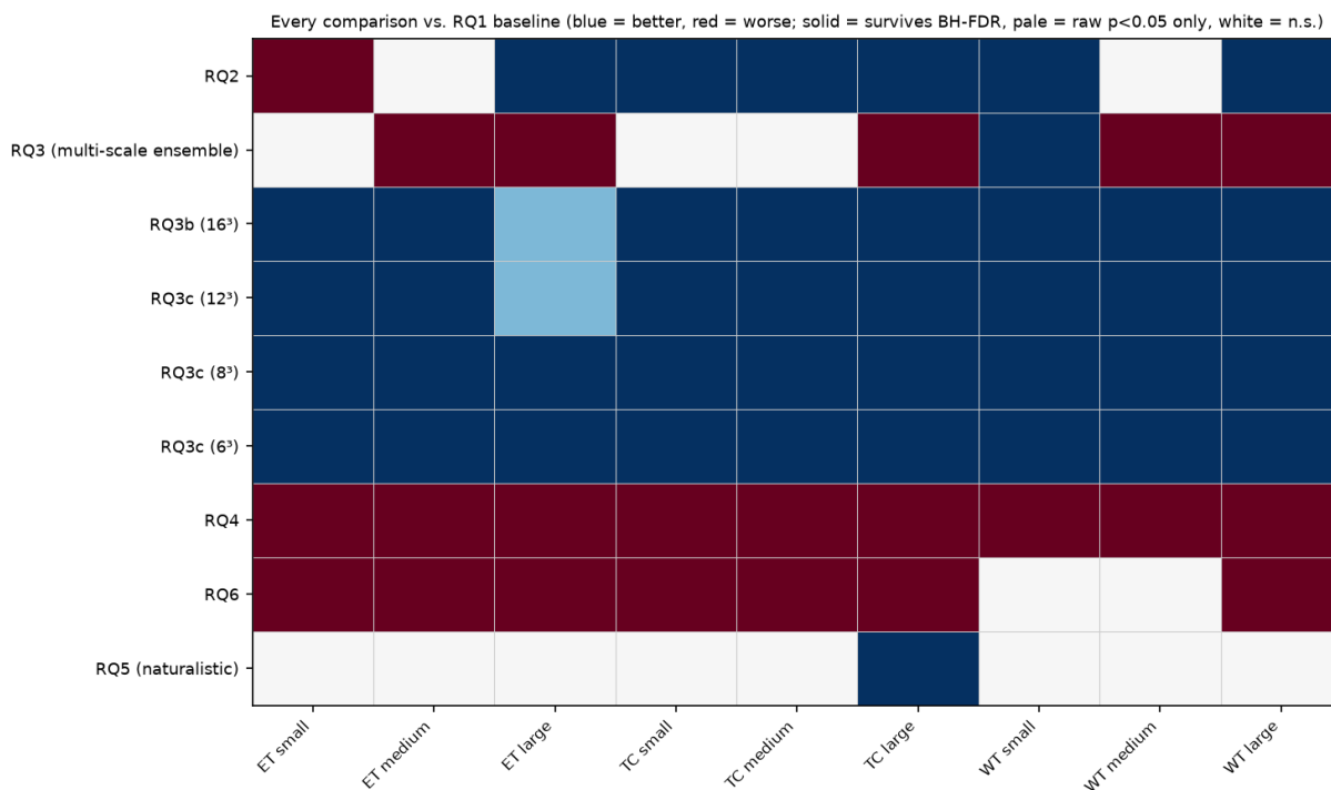
Figure 8: Every paired significance test run in this project, RQ1 baseline vs. each ablation, one row per comparison, one column per region×size bin. Blue = significantly better, red = significantly worse, white = no significant difference; solid color survives BH-FDR correction, pale color is significant only before correction.
