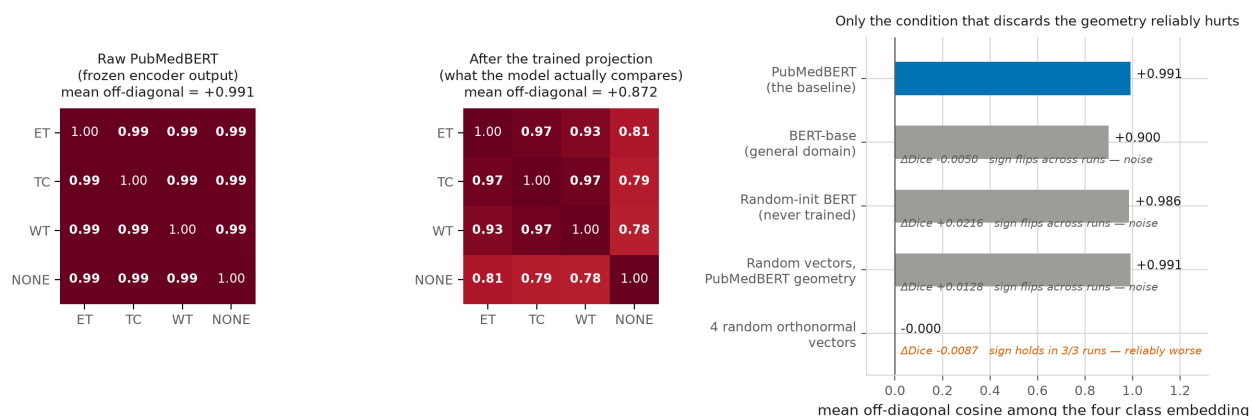
Figure 3: The single fact that makes the rest of this report interpretable. Left: the four class descriptions as PubMedBERT emits them, at 0.99 pairwise cosine — the frozen encoder barely distinguishes “enhancing tumor” from “no tumor”. Centre: the same four vectors after the trained linear head, which is where all of the separation is introduced (and even there, only the background class moves appreciably away). Right, previewing Section 7.8: every text condition RQ7 substitutes in, ordered by that same geometry statistic. The three conditions matching PubMedBERT’s anisotropic geometry are indistinguishable from retraining noise no matter what they mean; the one that discards it is the only one that reliably costs anything. Cosine matrices share a -1 to +1 colour scale.
