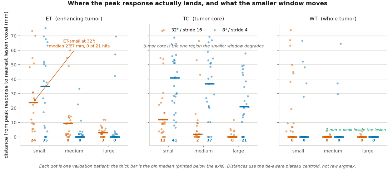
Figure 12: What the hit rate summarises. Each dot is one validation patient’s distance from the peak response to the nearest lesion voxel; the thick bar is the bin median. The ET-small failure is visible as a distribution, not a near miss — at 32^3 the peak sits a median 23.7 mm away with almost no mass at zero. The blue series previews Section 7.11: the 8^3 window pulls enhancing tumor down toward zero in every bin and pushes tumor core sharply away, a regional split Dice never showed.
