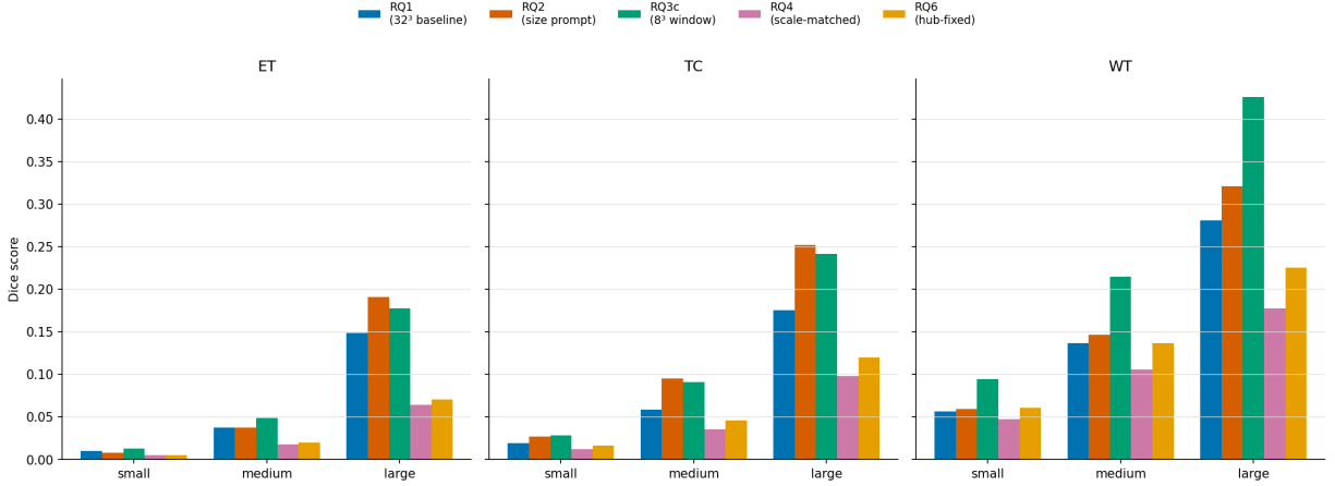
Figure 28: Leaderboard: every method’s mean Dice, one panel per region, bars grouped by size bin. These are Otsu-thresholded scores, the project’s original protocol; Section 7.11 shows the absolute values here understate the smaller-window arms and that Otsu is not a neutral common factor across them.
