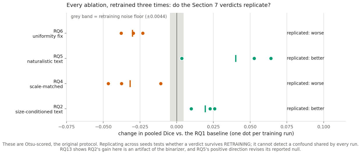
Figure 24: Each ablation retrained three times: one dot per run, tick at the mean, grey band the retraining noise floor.
