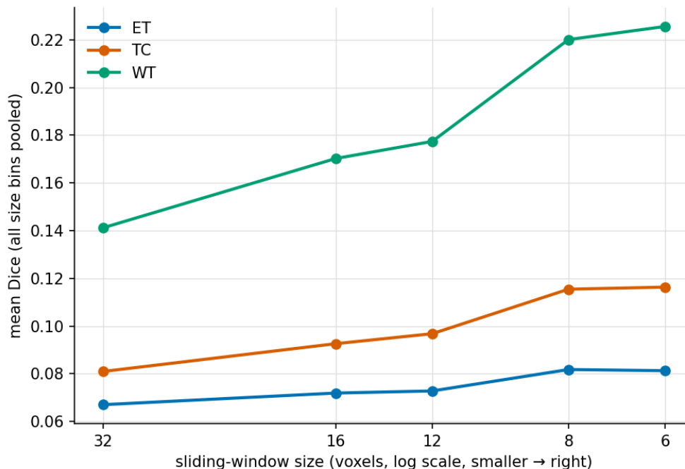
Figure 17: Mean Dice (pooled across size bins) vs. sliding-window size, one line per region. The trend from RQ3b continues through 12^3/8^3 , then plateaus for ET/TC at 6^3 while WT keeps climbing.
