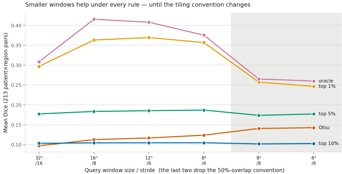
Figure 26: The window sweep re-scored under every binarization rule. Columns are window/stride; the first four hold the 50%-overlap convention fixed and the last two are the non-overlapping points the original sweep switched to. Only the Otsu curve keeps rising across that switch.
