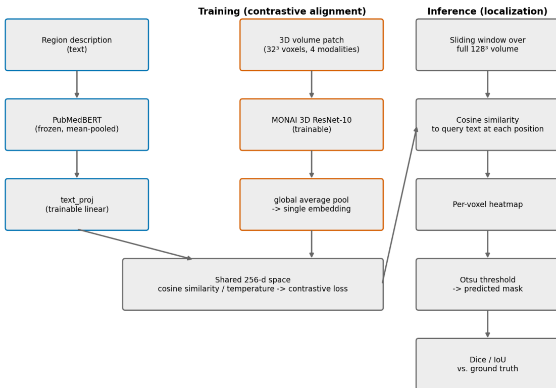
Figure 4: Pipeline schematic: contrastive text-volume alignment at training time (left/center), and sliding-window heatmap extraction at inference time (right).
