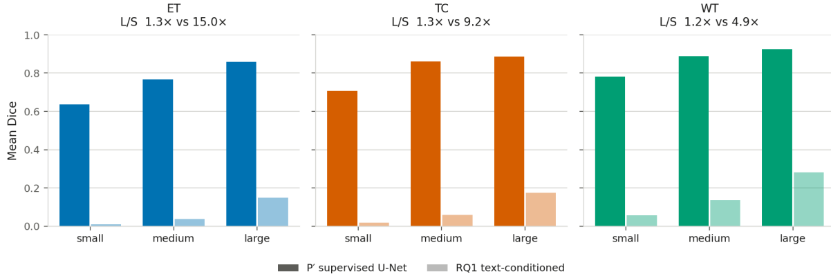
Figure 5: P' validation. Left to right: enhancing tumor, tumor core, whole tumor. Solid bars are the supervised U-Net, faded bars the text-conditioned baseline, both on the same held-out patients under the same Dice implementation. The supervised model’s large/small ratio is 1.2–1.3× against the text-conditioned 4.9–15.0×.
