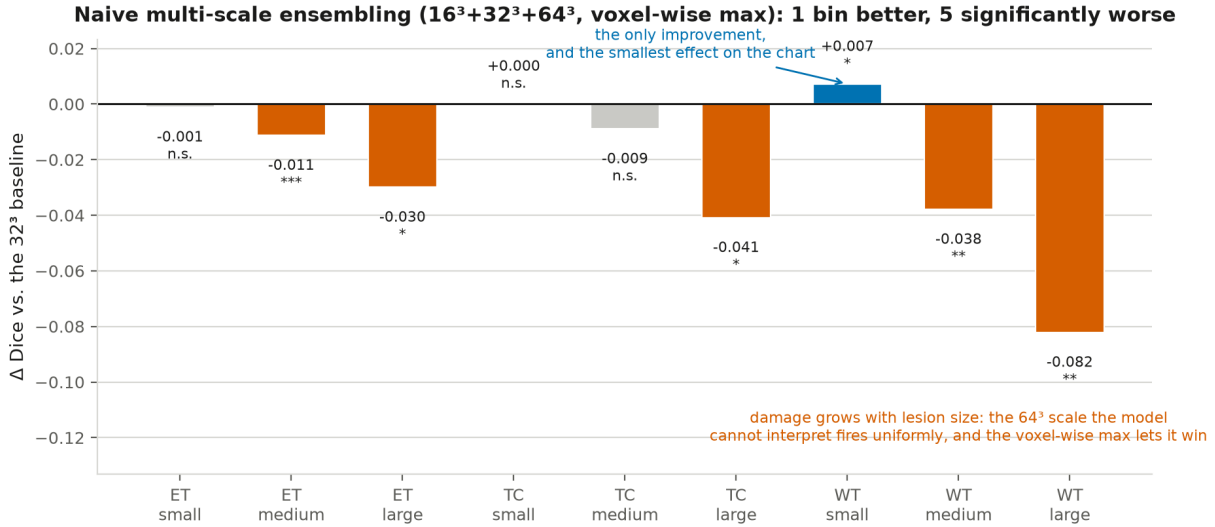
Figure 15: Naive multi-scale ensembling, per region and size bin, against the 32^3 baseline. Orange bars are significant losses after BH-FDR correction, grey are not significant, blue is the single improvement — which is also the smallest effect on the chart. The damage grows monotonically with lesion size within every region, which is the signature of a voxel-wise max importing noise from the 64^3 scale the model was never trained to interpret.
