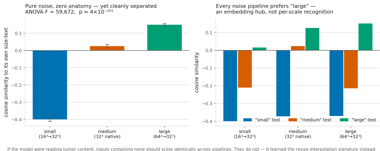
Figure 19: The RQ4 noise probe. Left: pure Gaussian noise containing no anatomy separates almost perfectly across the three resize pipelines. Right: the cross-check revealing a “large”-class hub rather than per-scale recognition.
