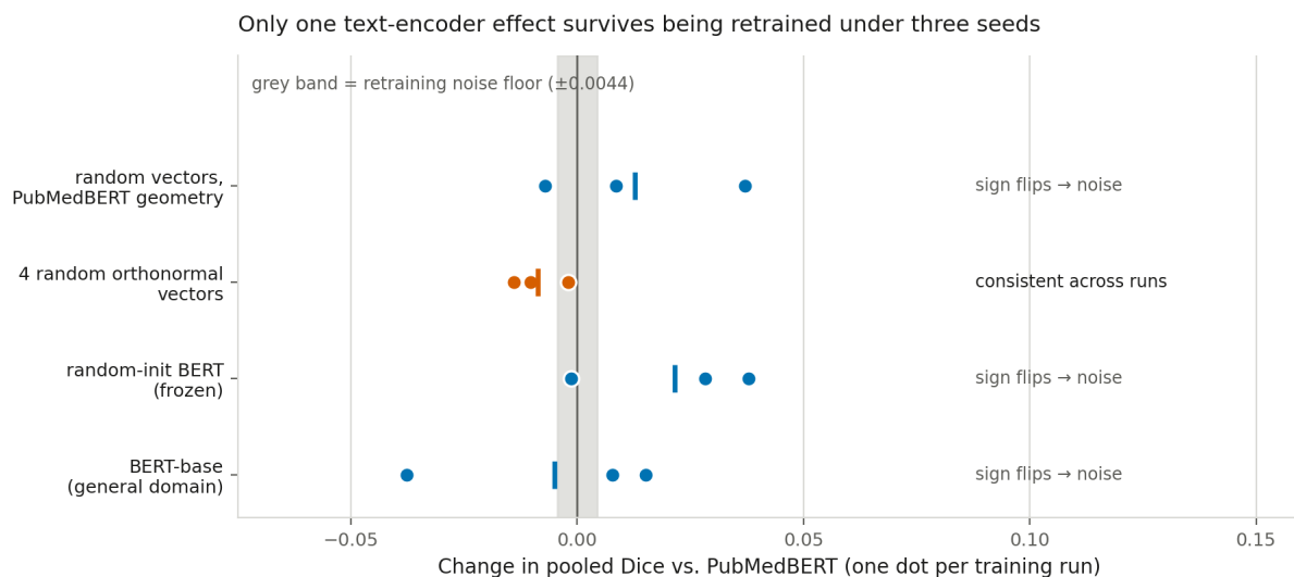
Figure 21: RQ7 text-encoder ablations. Each dot is one independent training run; the vertical tick is the mean of the three. The grey band is the retraining noise floor, measured by retraining the identical PubMedBERT baseline under three seeds. Only the orthonormal-vector condition (orange) keeps its sign across all three runs; the other three change direction from run to run despite within-run p-values as small as 6 \times 10^{-35} .
