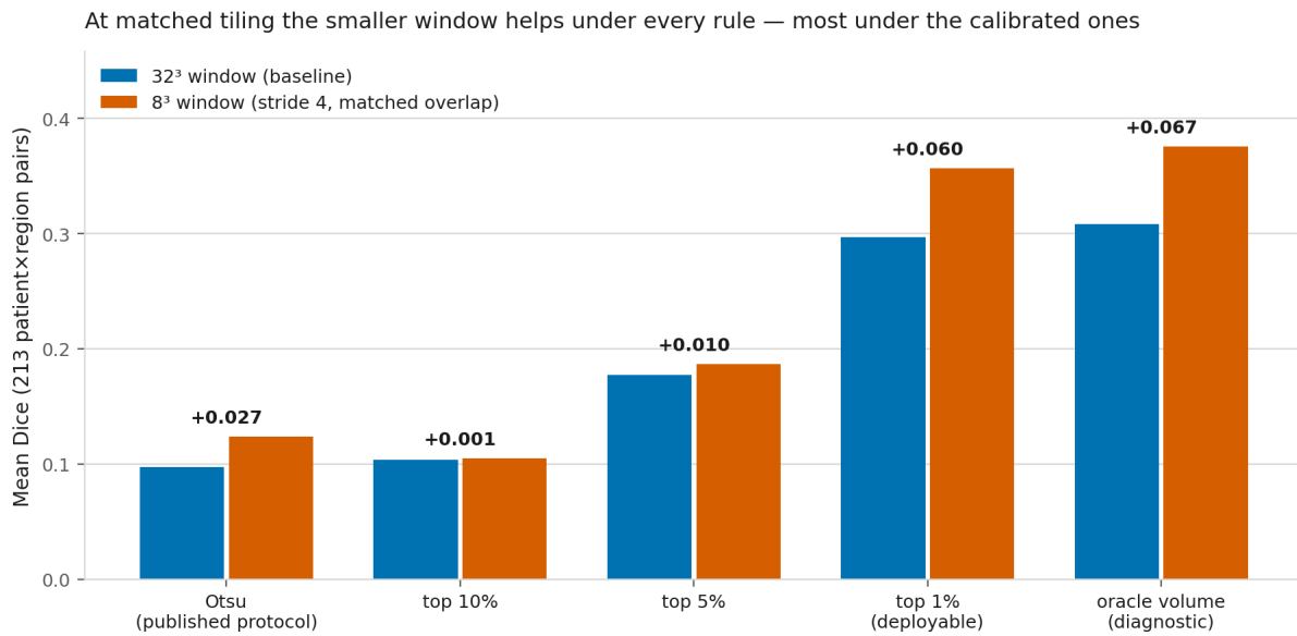
Figure 25: The 32 3 baseline against an 8 3 window at matched 50% overlap, on the same patients under the same Dice implementation. The advantage is real under every binarization rule and largest under the two that best reflect heatmap quality — the reverse of what the first, tiling-confounded version of this comparison showed.
