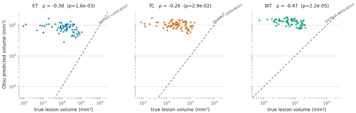
Figure 9: Otsu’s predicted mask volume against true lesion volume, log axes. A calibrated predictor would follow the dashed diagonal; instead predictions form a near-flat cloud two orders of magnitude above it, trending downward.
