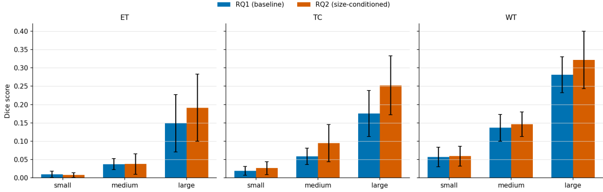
Figure 14: RQ1 (baseline) vs RQ2 (size-conditioned) Dice by region and size bin, error bars = 1 std.
