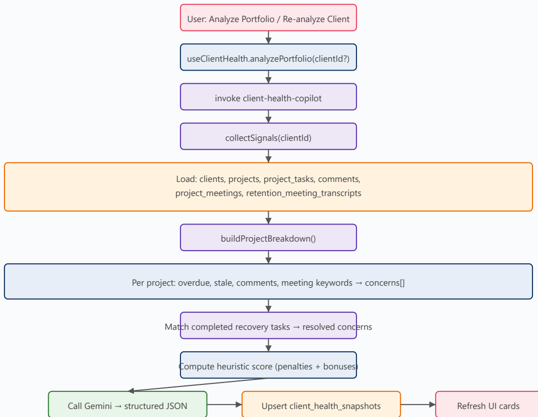
Figure 4 — Portfolio analysis sequence
