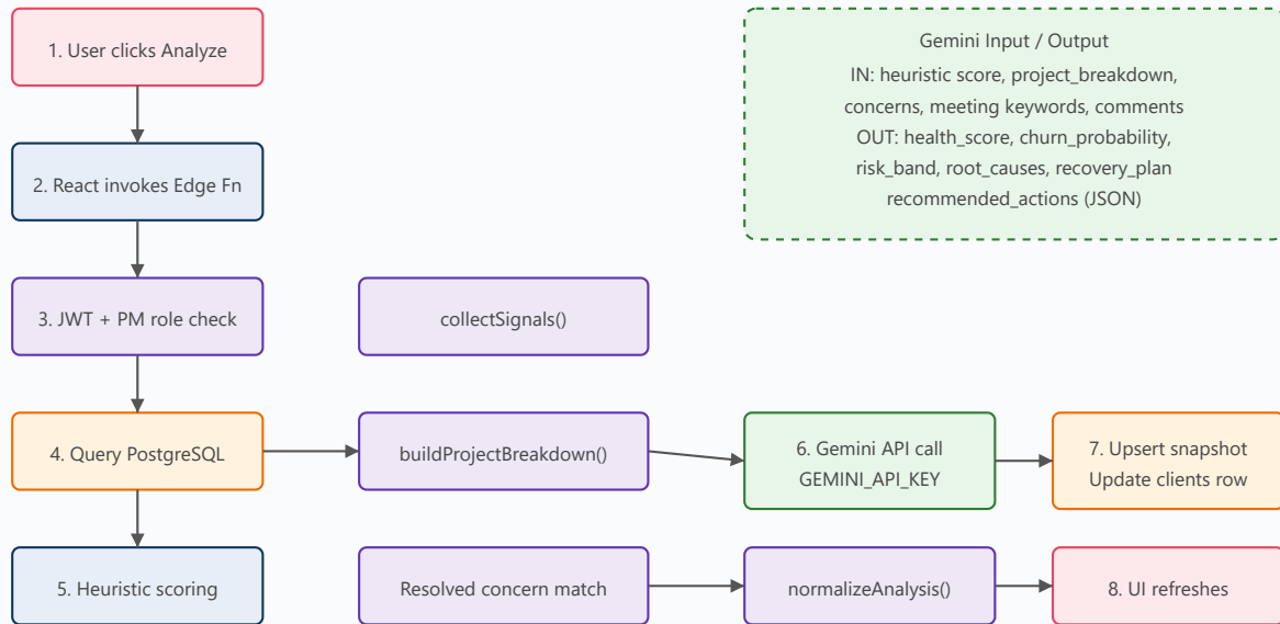
Figure 2 — Supabase + Gemini AI integration flow
