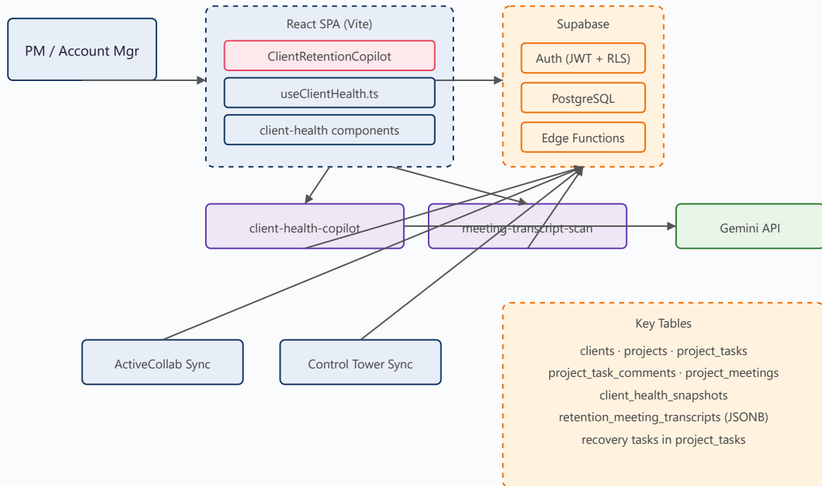
Figure 1 — End-to-end system context
