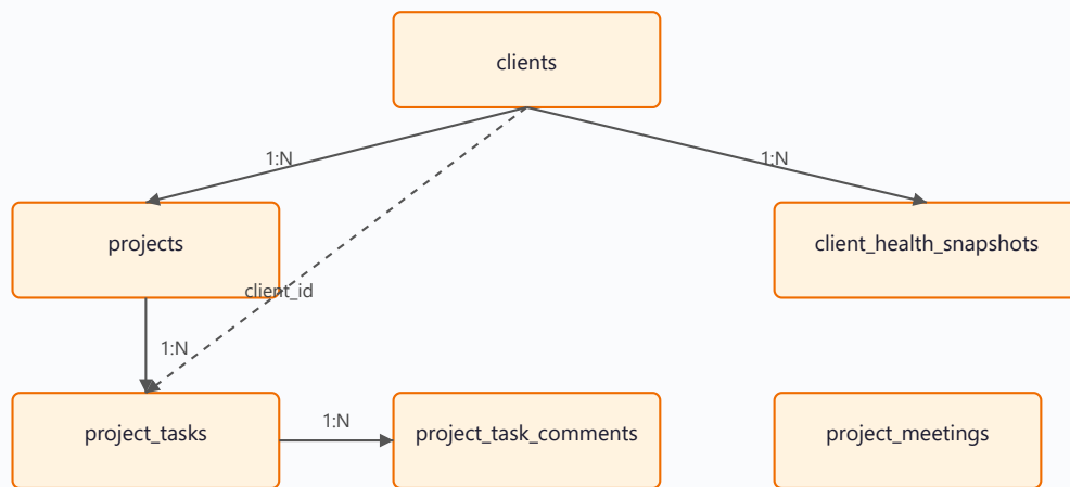
Figure 3 — Entity relationships
