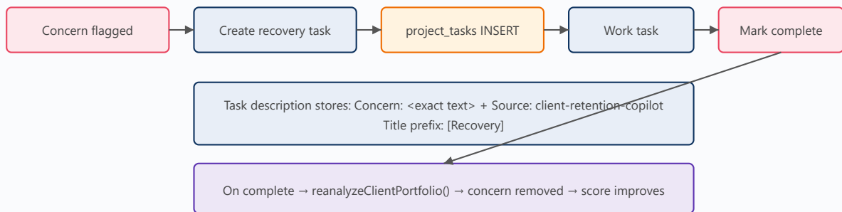
Figure 6 — Concern → recovery task → score revision
