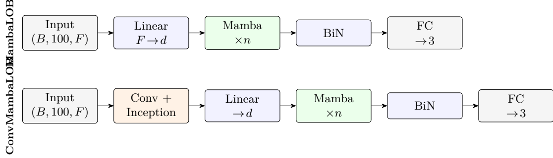
Figure 1: Proposed architectures. MambaLOB (top) projects the LOB vector and applies n selective state-space blocks ( O(L) temporal mixing) before Bilinear Normalization and a 3-class head. ConvMambaLOB (bottom) prepends DeepLOB’s Conv + Inception spatial extractor, replacing DeepLOB’s sequential LSTM with the Mamba core. Bidirectional and combined variants were also evaluated (Section 3.6).
