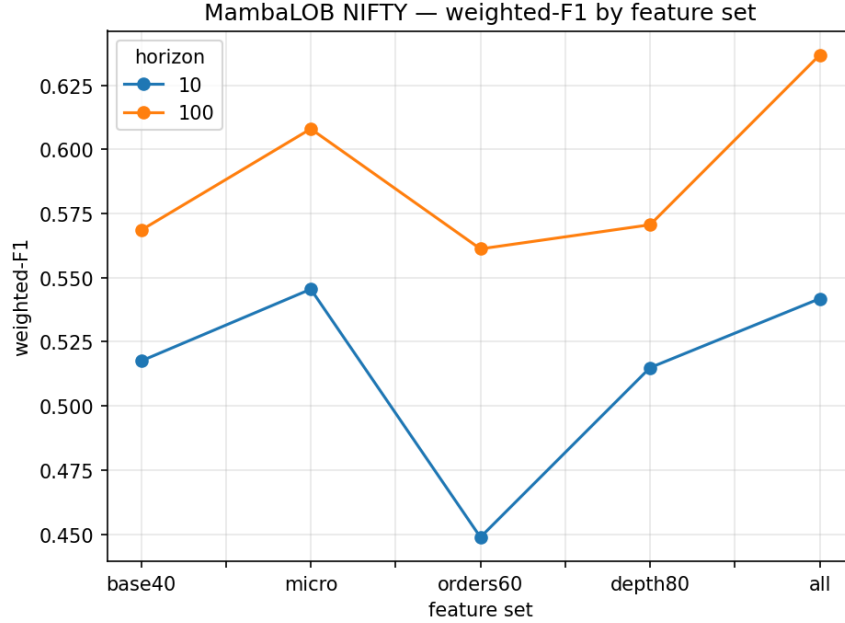
Figure 3: MambaLOB (NIFTY) weighted- F_1 by feature set and horizon. The engineered micro and all sets sit above raw base40 , with the gain widening at the longer horizon; deep levels ( depth80 ) and order counts alone ( orders60 ) do not help in isolation.
