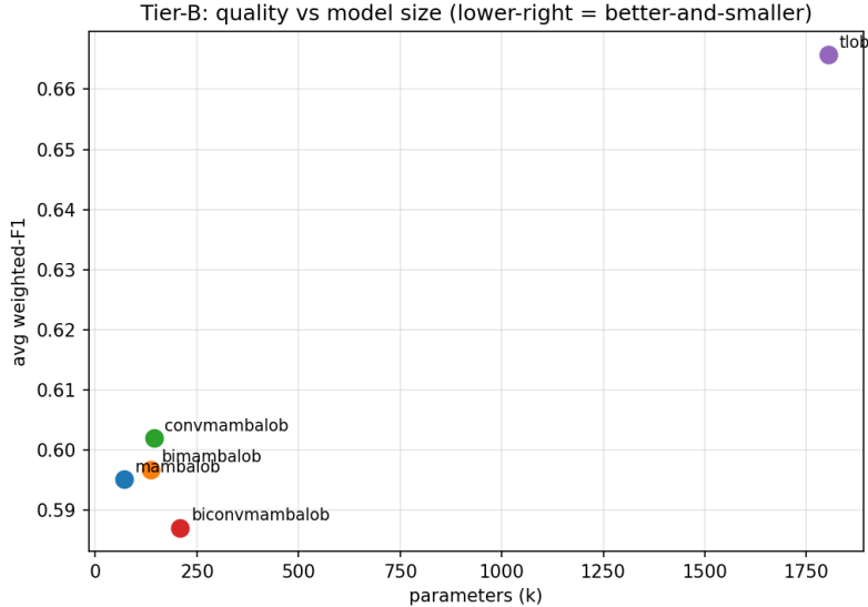
Figure 7: Quality vs. model size for the Tier-B architectures (average weighted- F_1 against parameter count). The Mamba family clusters at the low-parameter end near TLOB’s accuracy; ConvMambaLOB is the best of the proposed variants. The lower-right region (better-and-smaller) is the design target.
