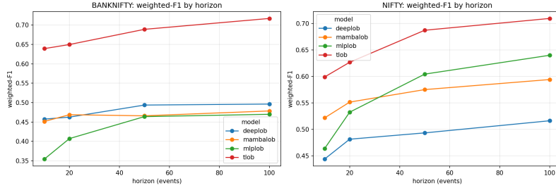
Figure 6: NSE transfer (Scheme A): test weighted- F_1 by horizon for each model. TLOB leads throughout; MambaLOB transfers competitively, matching or beating the CNN baseline on NIFTY at a fraction of the parameters.
