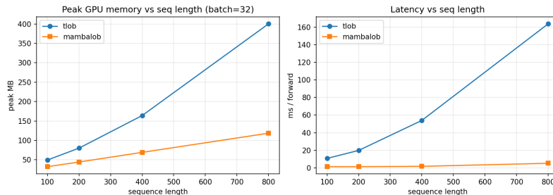
Figure 8: Sequence-length scaling: TLOB’s O(L^2) attention versus MambaLOB’s O(L) selective scan. The gap widens sharply with L , the basis of the architecture’s efficiency claim.
