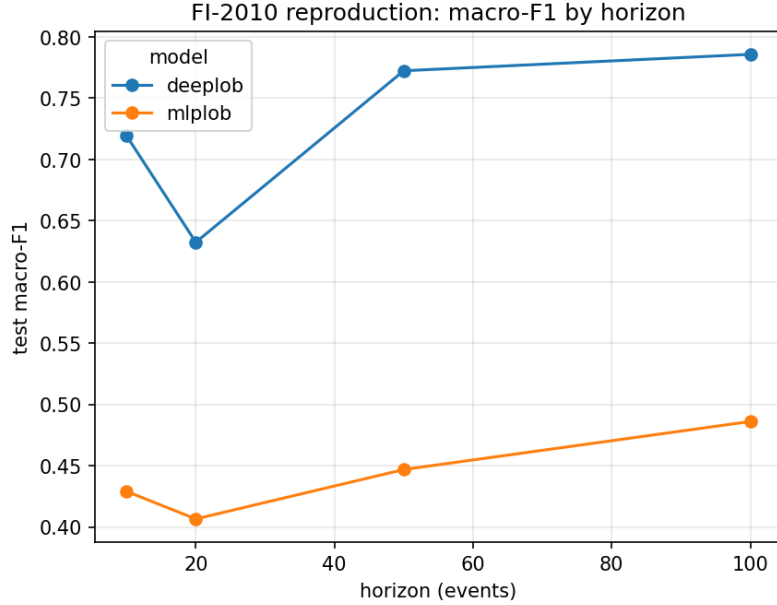
Figure 4: FI-2010 reproduction: macro- F_1 by prediction horizon for the reproduced baselines. The ordering and absolute range match the published DeepLOB/TLOB results and the independent LOBCAST reproduction.
