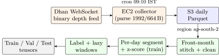
Figure 2: Engineered NSE data pipeline. The reverse-engineered Dhan binary feed (two frame formats, 1992 B full / 664 B compact) is parsed on an EC2 collector and written as daily Parquet to S3; the modelling layer then stitches the front-month series across the expiry roll, cleans, segments per trading day, z-scores using training statistics only, labels, and emits lazily-windowed tensors aligned to the FI-2010 layout.
