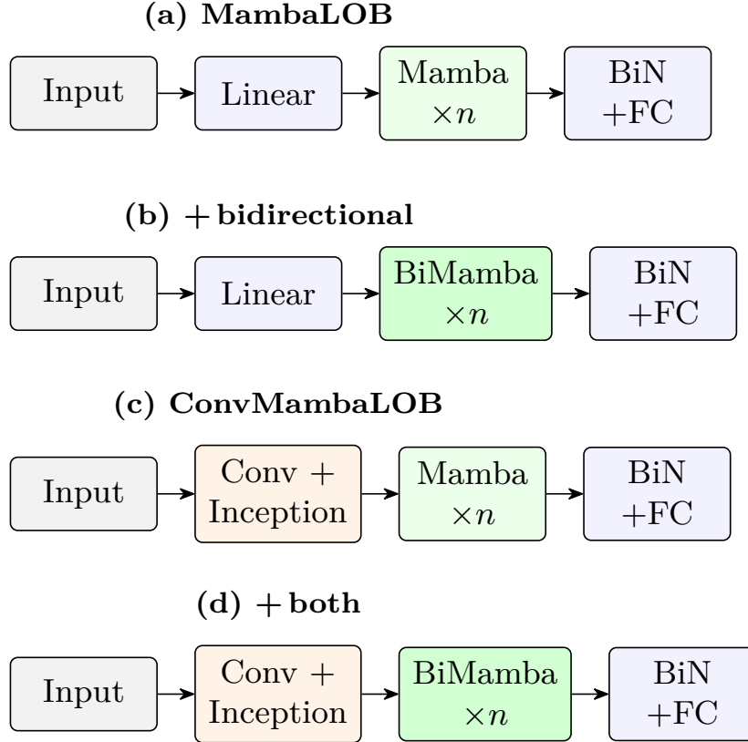
Figure 9: The four Tier-B variants. (a) base MambaLOB; (b) bidirectional Mamba (forward + time-reversed scan, averaged); (c) ConvMambaLOB (spatial conv front-end \rightarrow Mamba core); (d) both combined. All share the Bilinear-Normalization head. Variant (c) was the best of the four; (d) the weakest (Table 8).
