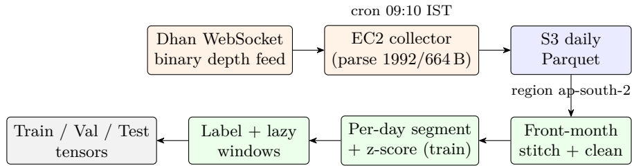
Figure 7: Engineered NSE data pipeline. The reverse-engineered Dhan binary feed (two frame formats, 1992B full / 664B compact) is parsed on an EC2 collector and written as daily Parquet to S3; the modelling layer then stitches the front-month series across the expiry roll, cleans, segments per trading day, z-scores using training statistics only, labels, and emits lazily-windowed tensors aligned to the FI-2010 layout.
