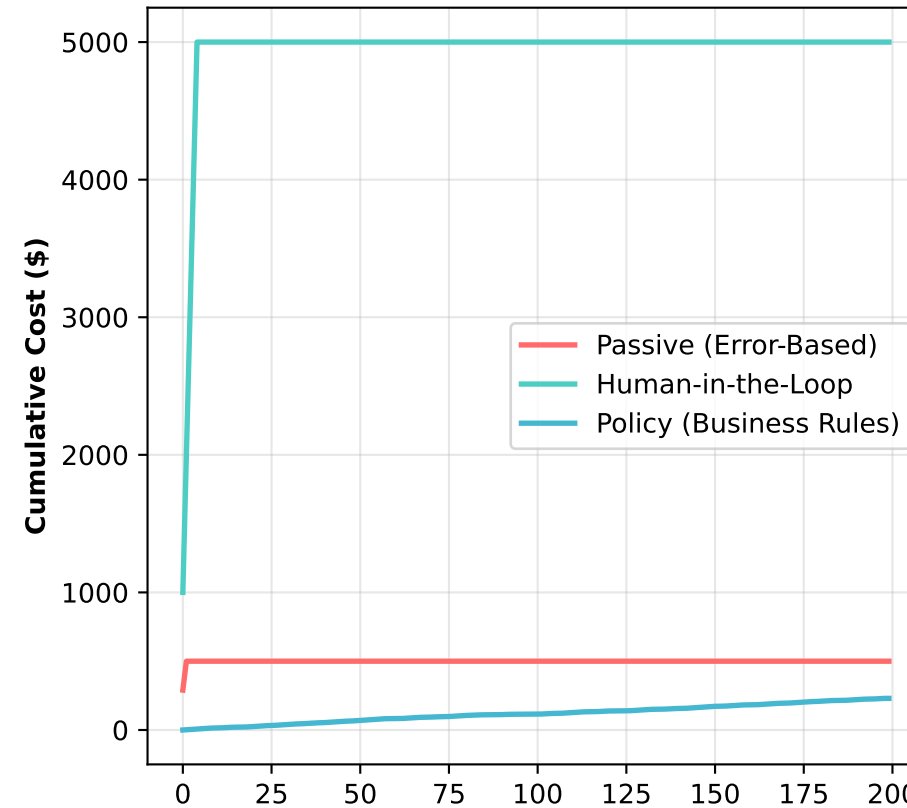
Feedback Cost Accumulation
