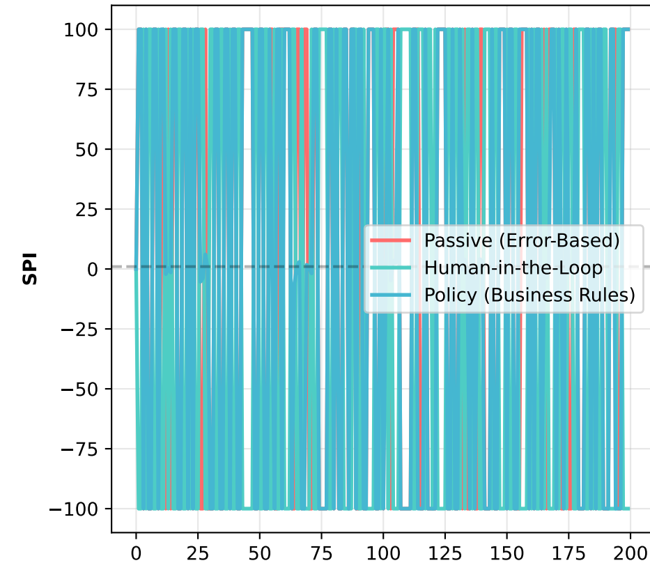
Stability-Plasticity Index
