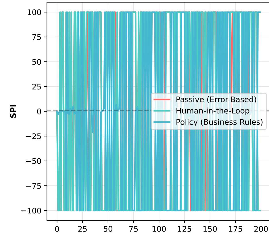
Stability-Plasticity Index
