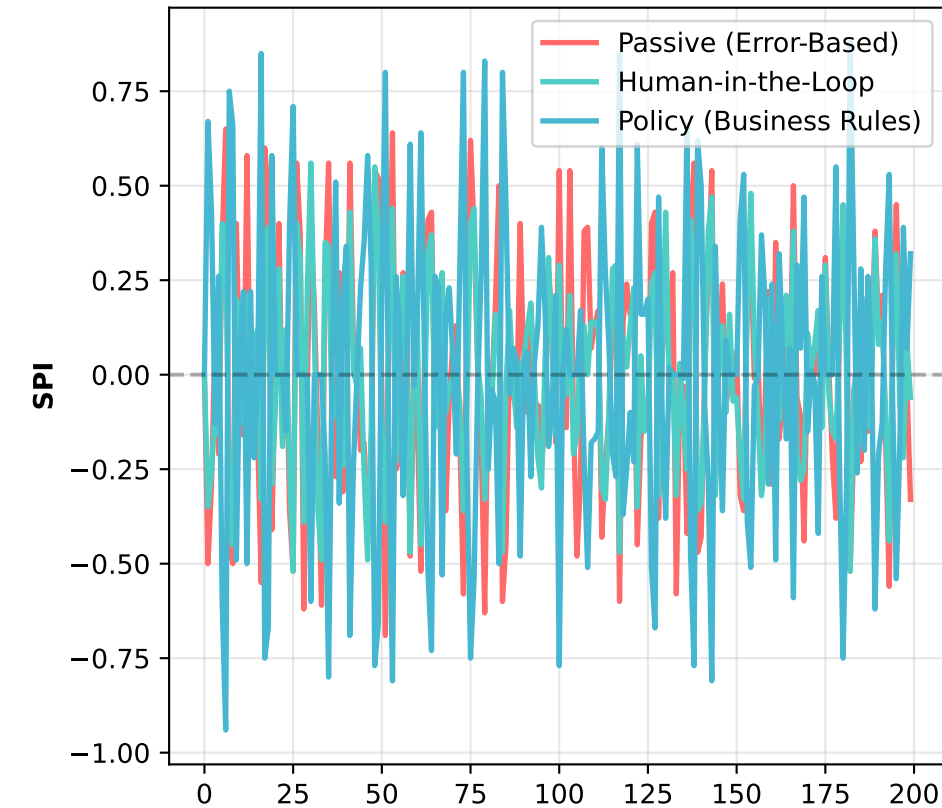
Stability-Plasticity Index
