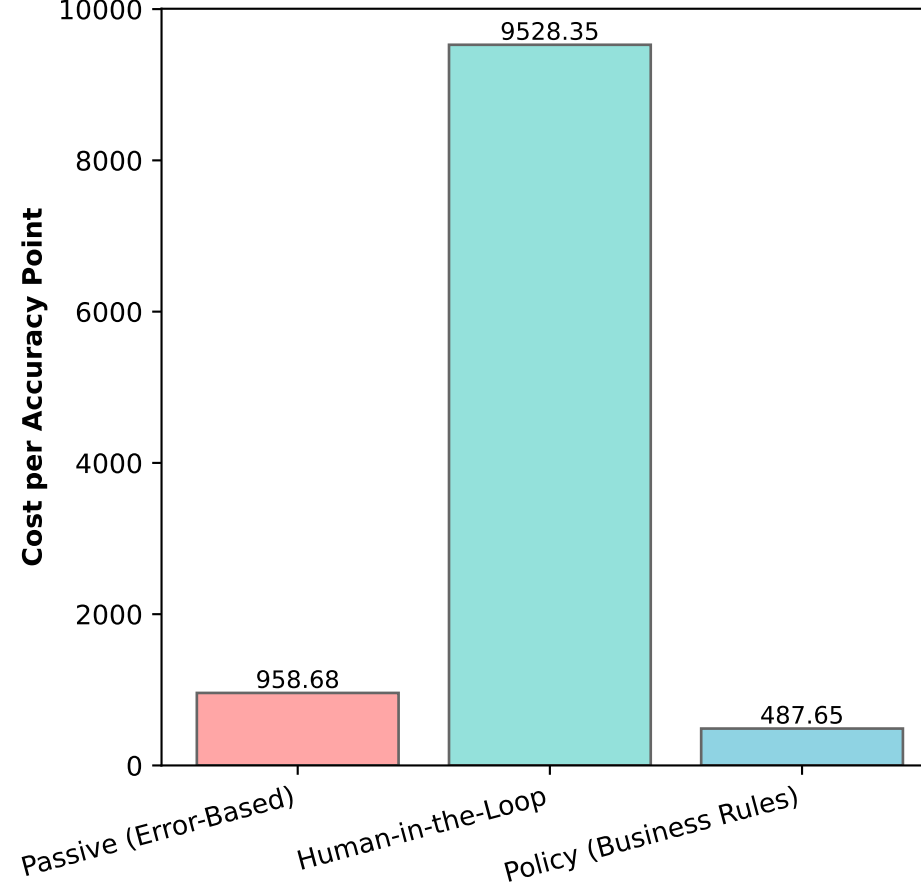
Feedback Efficiency (Lower is Better)
