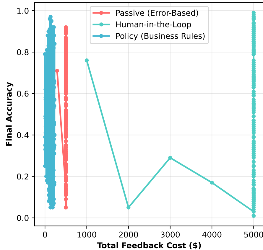
Accuracy-Cost Trade-Off (Pareto)
