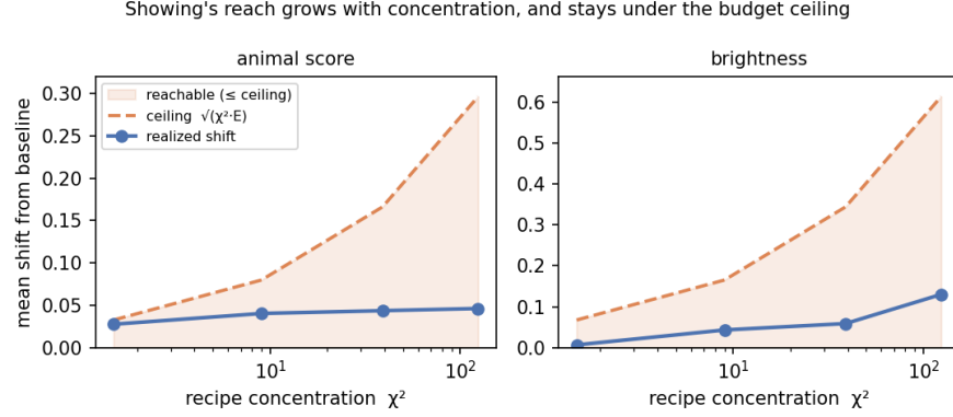
Figure 7: Claim 2: as the recipe concentrates ( \chi^2 rising), showing's realized shift grows and stays under the budget's ceiling \sqrt{\chi^2 \cdot E} . The ceiling climbs faster, so the cap is loose at high concentration; for brightness the model also falls short of the shift the budget allows.
