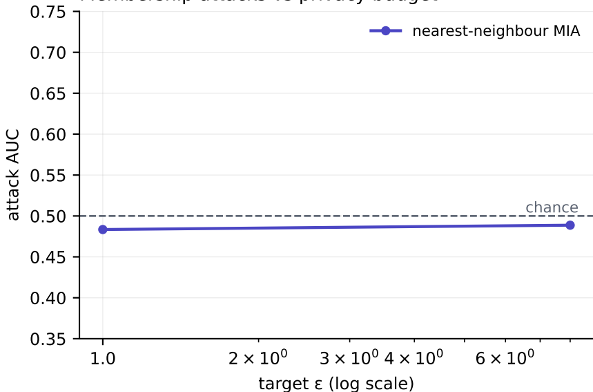
Membership attacks vs privacy budget
