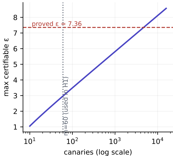
Audit ceiling
