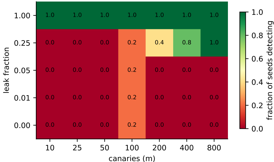
Auditor detection rate against known leakage
