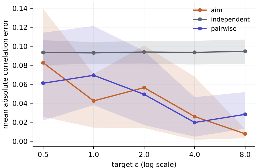
Structure preservation vs privacy budget
