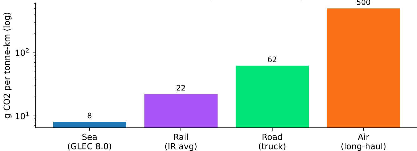
Pinned emission factors by mode (validate-gate enforced)
