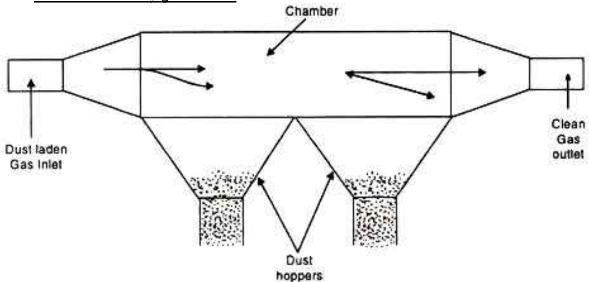
Fig. 6.4. Horizontal Flow Settling Chamber.
