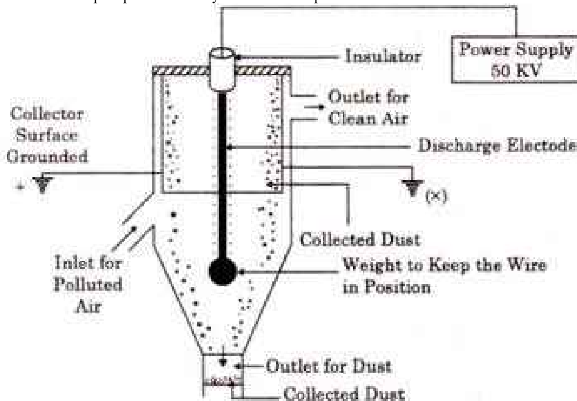
Fig. 5.4 Electrostatic Precipitator
