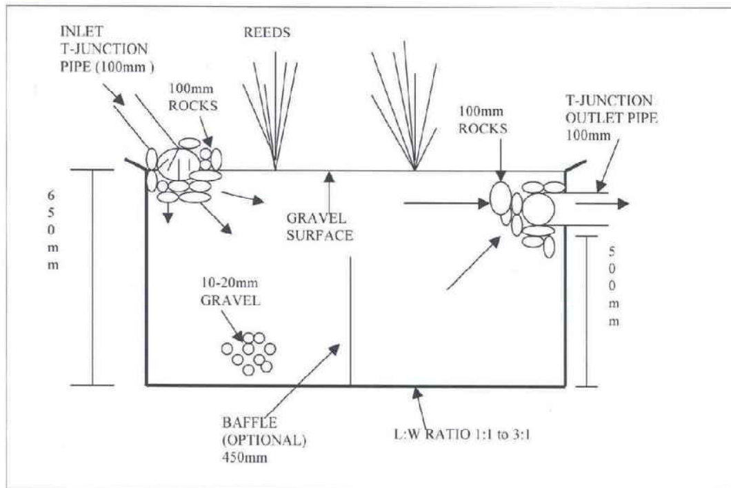
Figure : Basic Reed bed Design (Lateral View)
