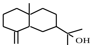
Eudesmol
