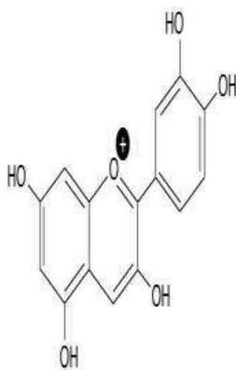
Cyanidin
