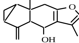
Linderene
