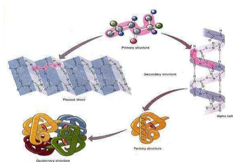
FIGURE 2-7 Models of the primary, secondary, tertiary, and quaternary structures of a protein. The secondary structure may consist of coils, alpha helices or folds (pleated sheets), depending on which amino acids form hydrogen bonds with each other.
