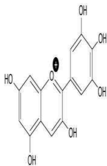
Delphinidin
