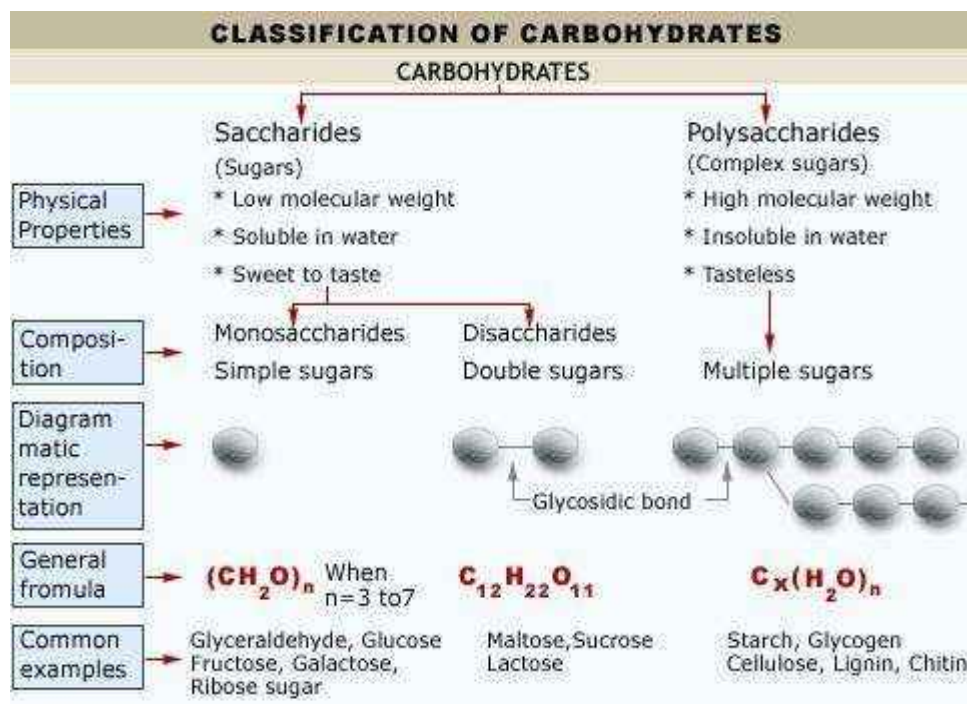
Classification of carbohydrates
