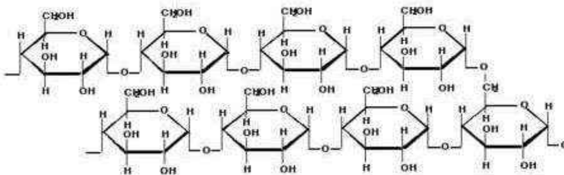
\alpha (1 \rightarrow 6) linkage at crosslink
