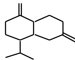
Bulgarene
