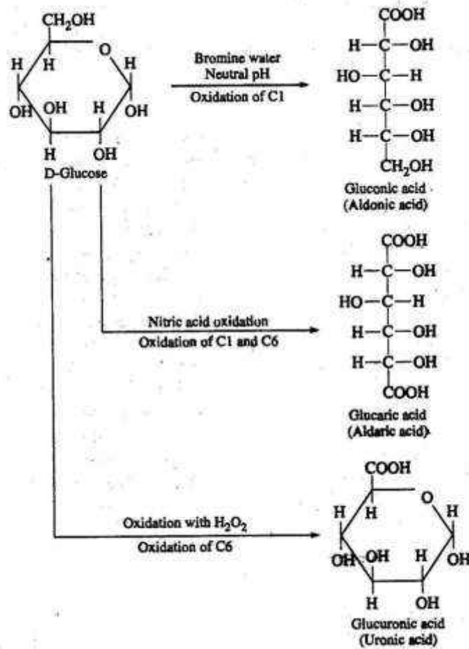
Oxidation products of glucose
