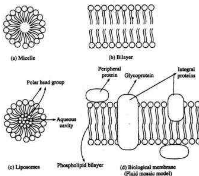
Structures of micelle, bilayer, liposome and biological membrane
