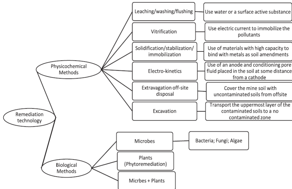
Fig. 1. Remediation technologies of metals in mine soils
