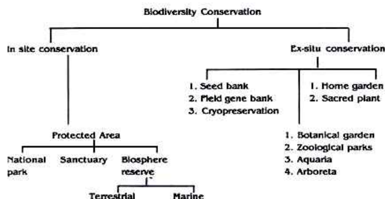
FIG. 5.1 : SCHEME SHOWING BIODIVERSITY CONSERVATION MANAGEMENT SYSTEMS.
