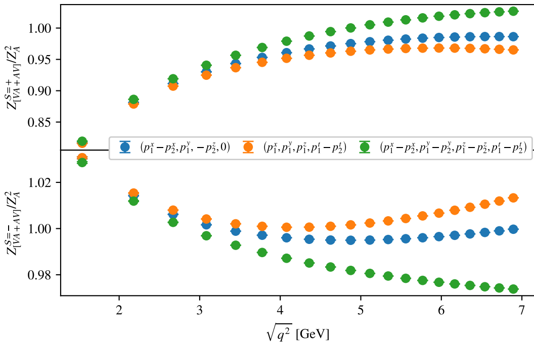
SMOM ^{\gamma_\mu} , m_\pi=0 , all combos
