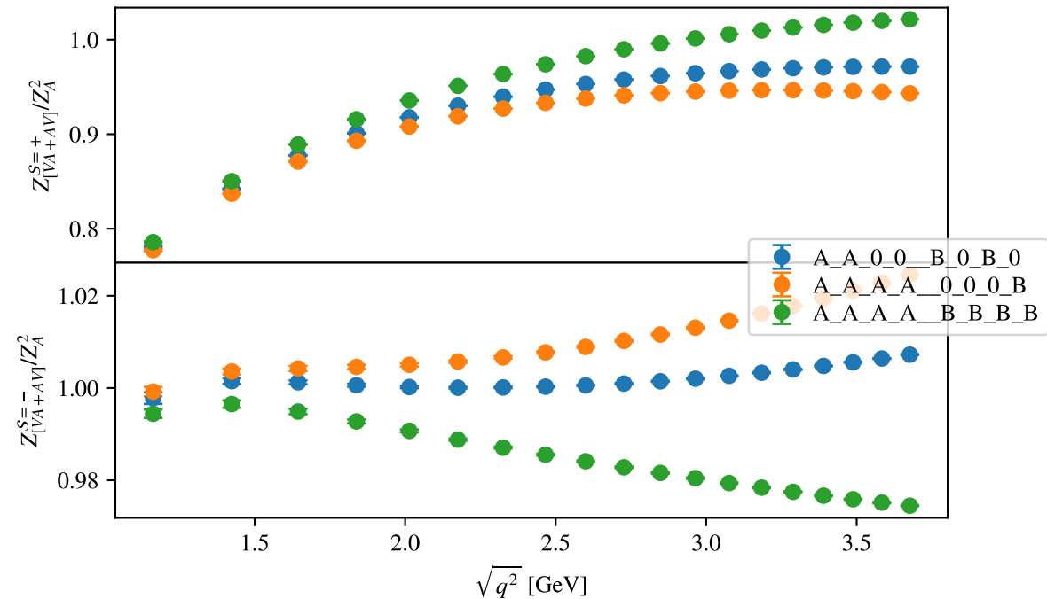
SMOM ^{\gamma_\mu} , m_\pi=0 , all combos
