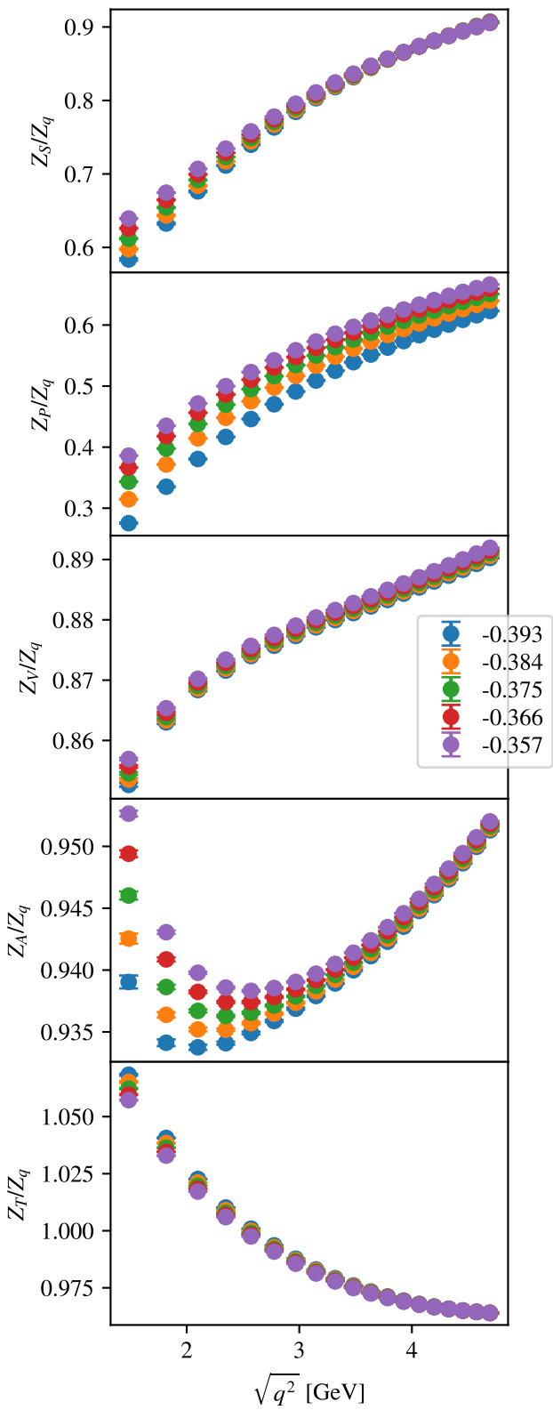
MOM ^{\gamma_\mu} , mom combo 2
