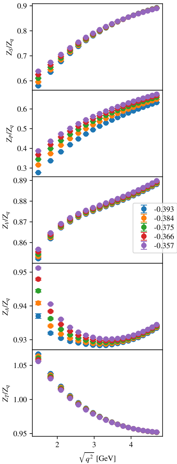
MOM ^{\gamma_\mu} , mom combo 5
