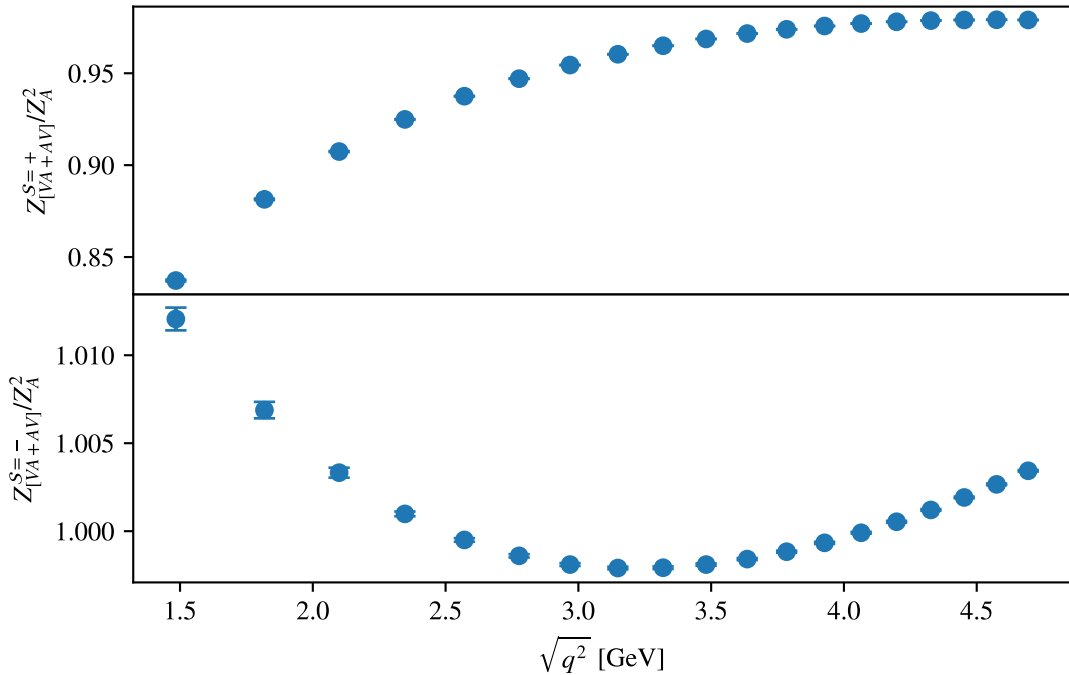
SMOM ^{\gamma_\mu} , m_\pi=0 mom combo 1
