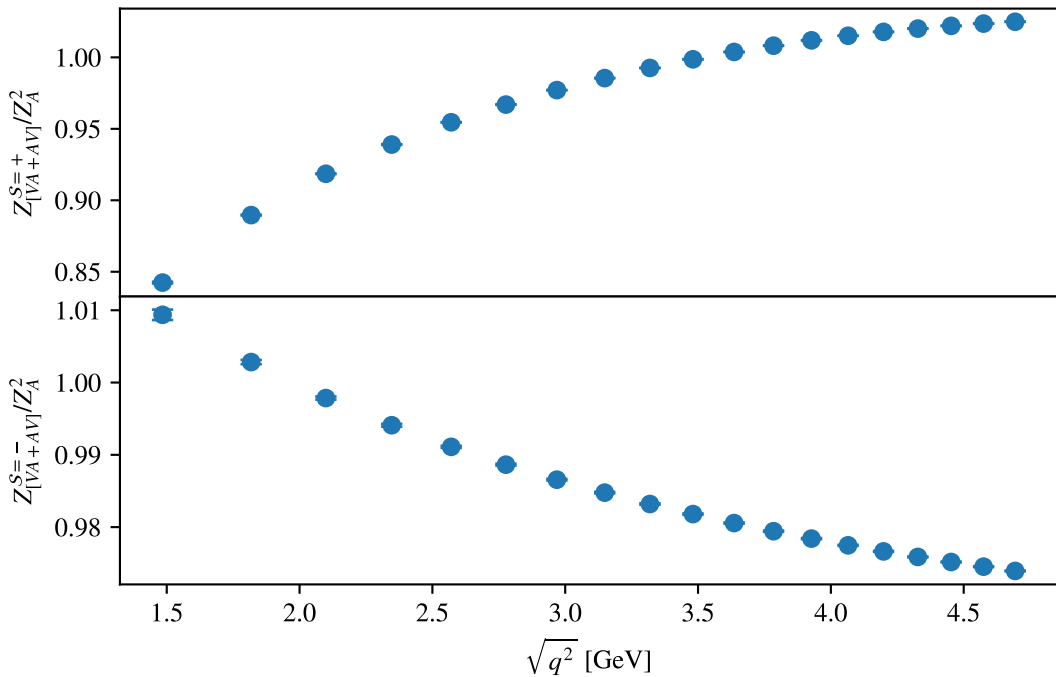
SMOM ^{\gamma_\mu} , m_\pi = 0 mom combo 3
