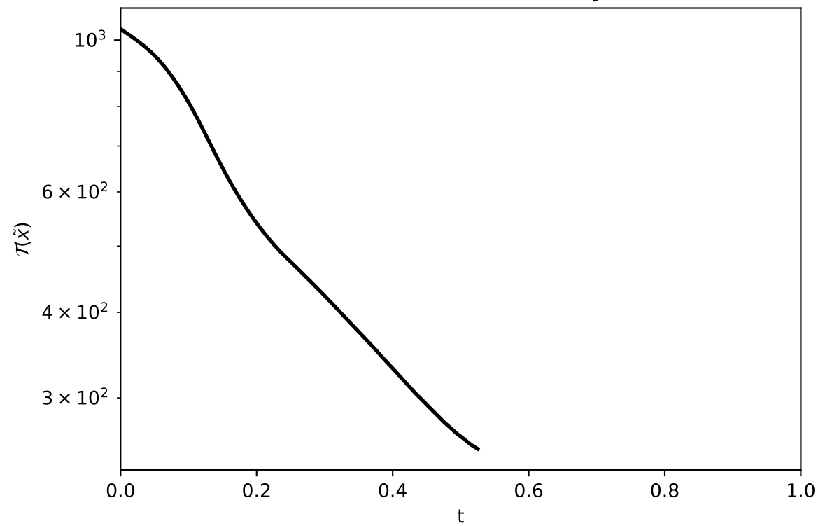
Terminal cost (CLF) decay
