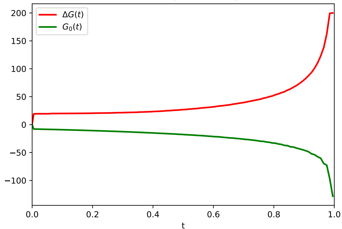
Terminal cost (CLF) decay
