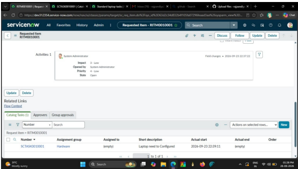
Requested Item: linked Catalog Task and Hardware assignment group.
