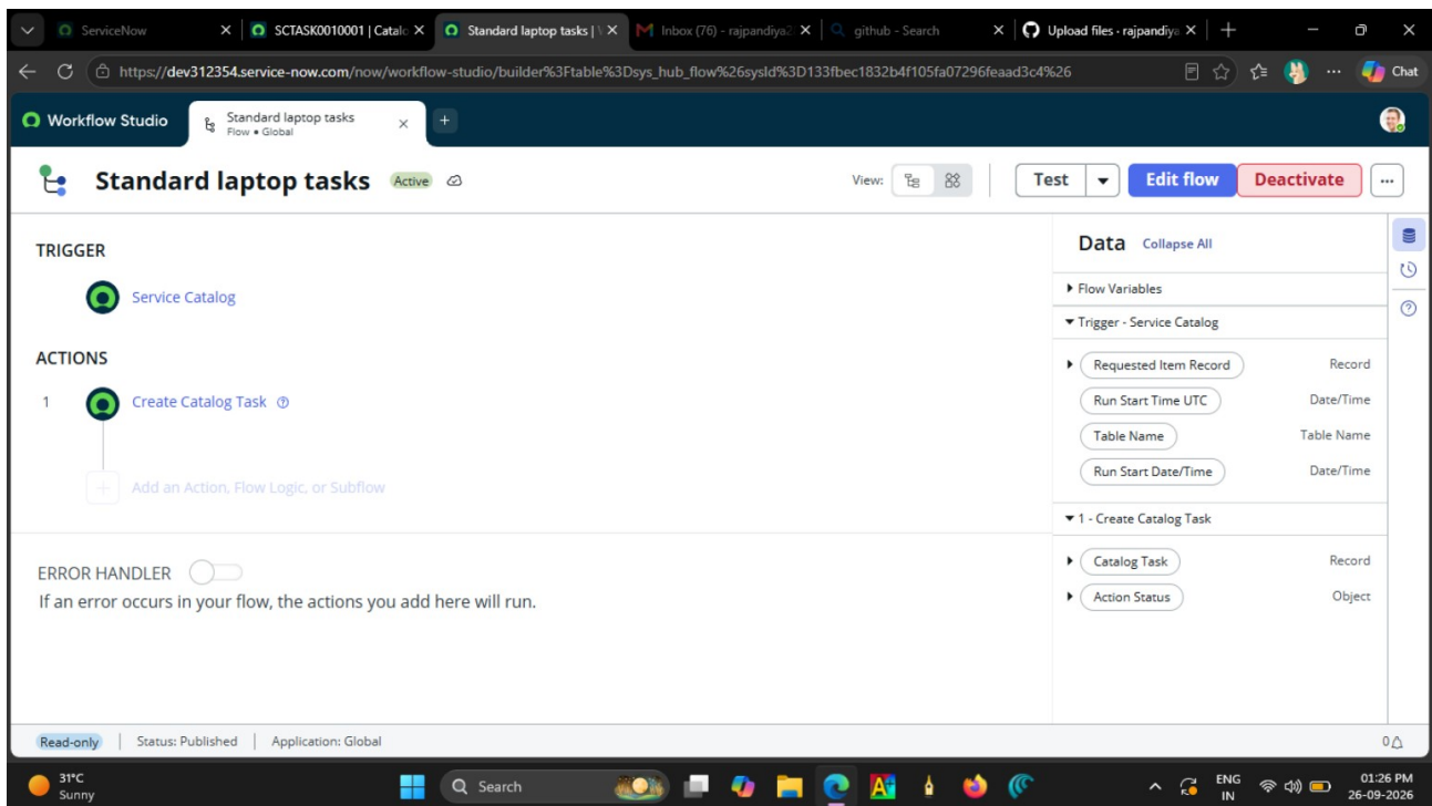
Figure: ServiceNow Flow Designer showing the Service Catalog trigger and Create Catalog Task action.
