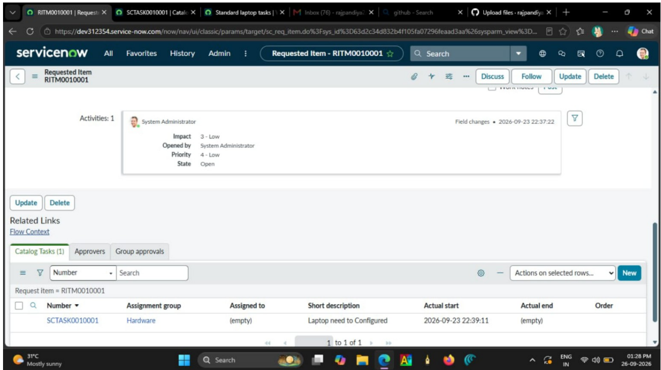
Figure 3. Requested Item with generated Catalog Task SCTASK0010001.
