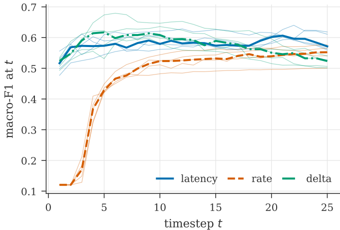
(a) NSL-KDD, every seed shown
