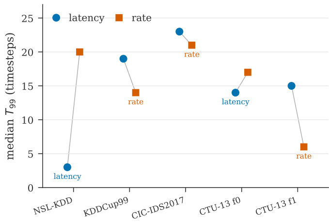
(b) convergence step, all strict protocols
